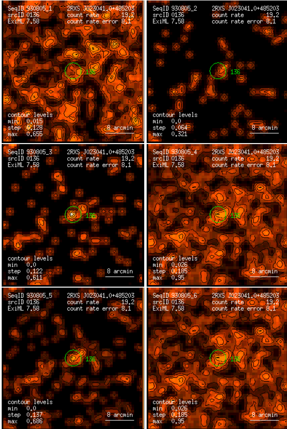
Figure 136: RASS 930805: detection 0136: band rate images, Gaussian filter: (1) PSPC channels 11 – 41, (2) 52 – 90, (3) 91 – 201, (4) 11 – 235, (5) 52 – 201, (6) 11 – 201. Broad band rates in counts/ks. Band rate contour levels in counts/ks/arcmin 2 .
