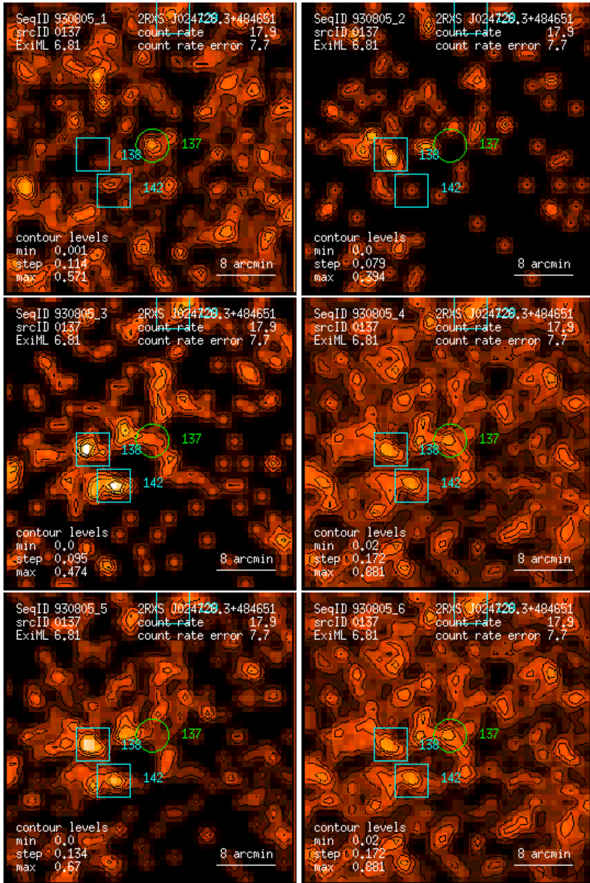
Figure 137: RASS 930805: detection 0137: band rate images, Gaussian filter: (1) PSPC channels 11 – 41, (2) 52 – 90, (3) 91 – 201, (4) 11 – 235, (5) 52 – 201, (6) 11 – 201. Broad band rates in counts/ks. Band rate contour levels in counts/ks/arcmin 2 .
