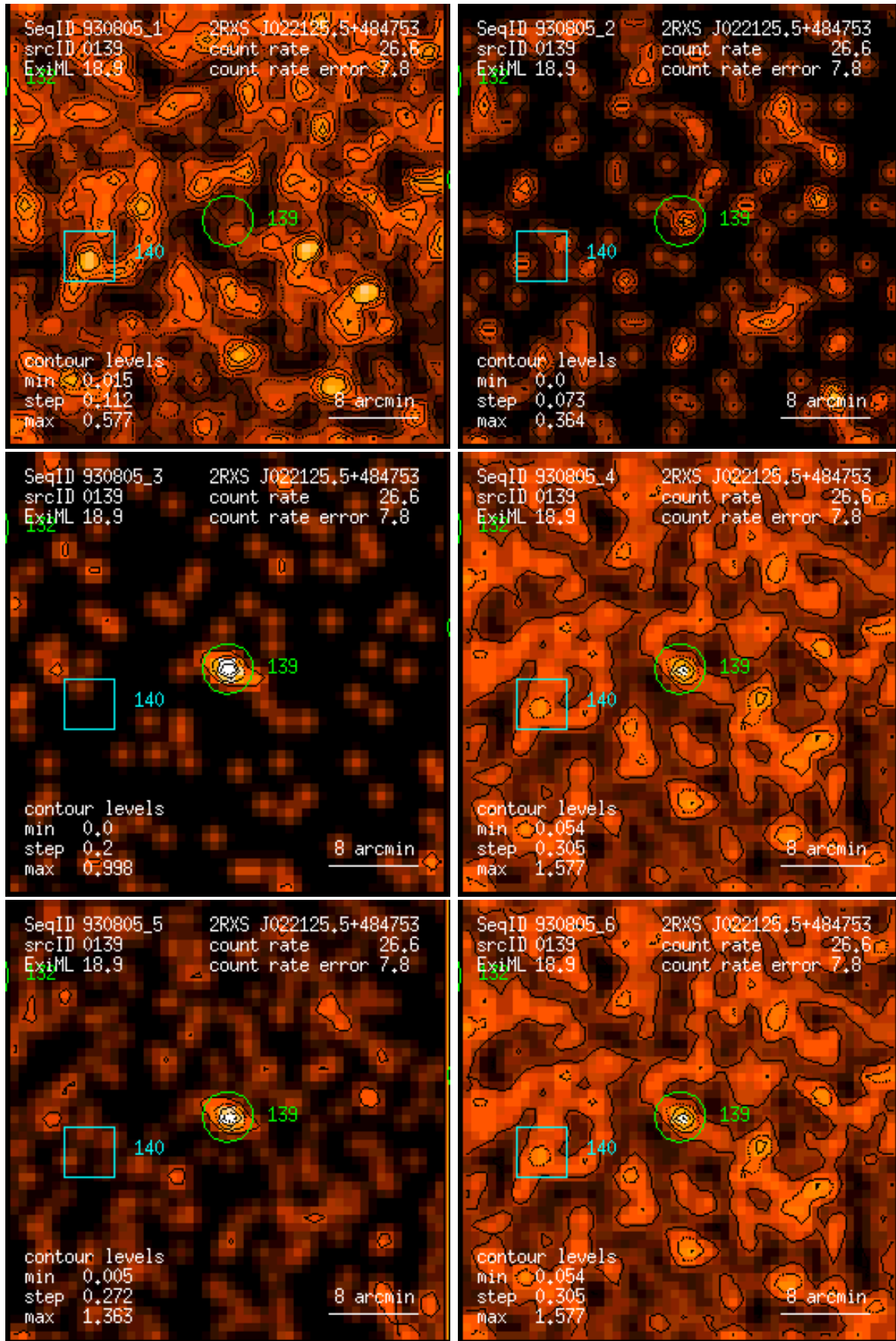
Figure 139: RASS 930805: detection 0139: band rate images, Gaussian filter: (1) PSPC channels 11 – 41, (2) 52 – 90, (3) 91 – 201, (4) 11 – 235, (5) 52 – 201, (6) 11 – 201. Broad band rates in counts/ks. Band rate contour levels in counts/ks/arcmin 2 .
