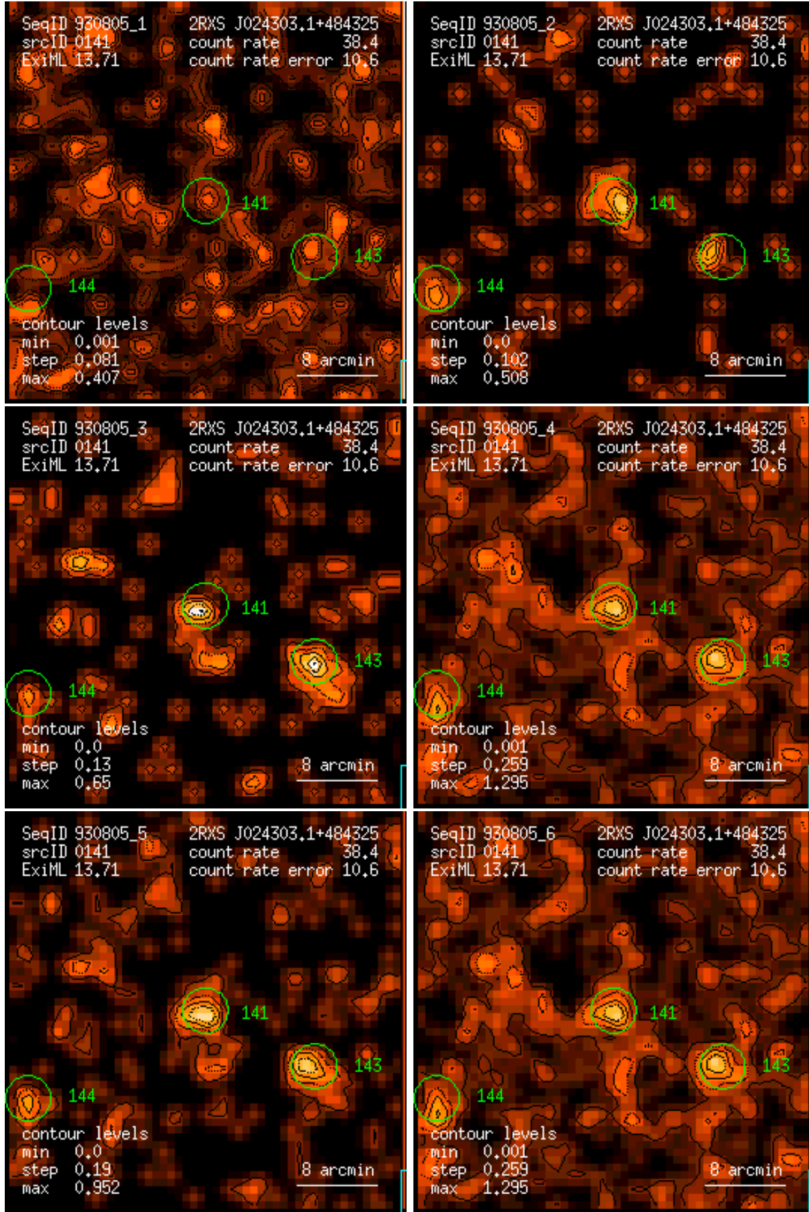
Figure 141: RASS 930805: detection 0141: band rate images, Gaussian filter: (1) PSPC channels 11 – 41, (2) 52 – 90, (3) 91 – 201, (4) 11 – 235, (5) 52 – 201, (6) 11 – 201. Broad band rates in counts/ks. Band rate contour levels in counts/ks/arcmin 2 .
