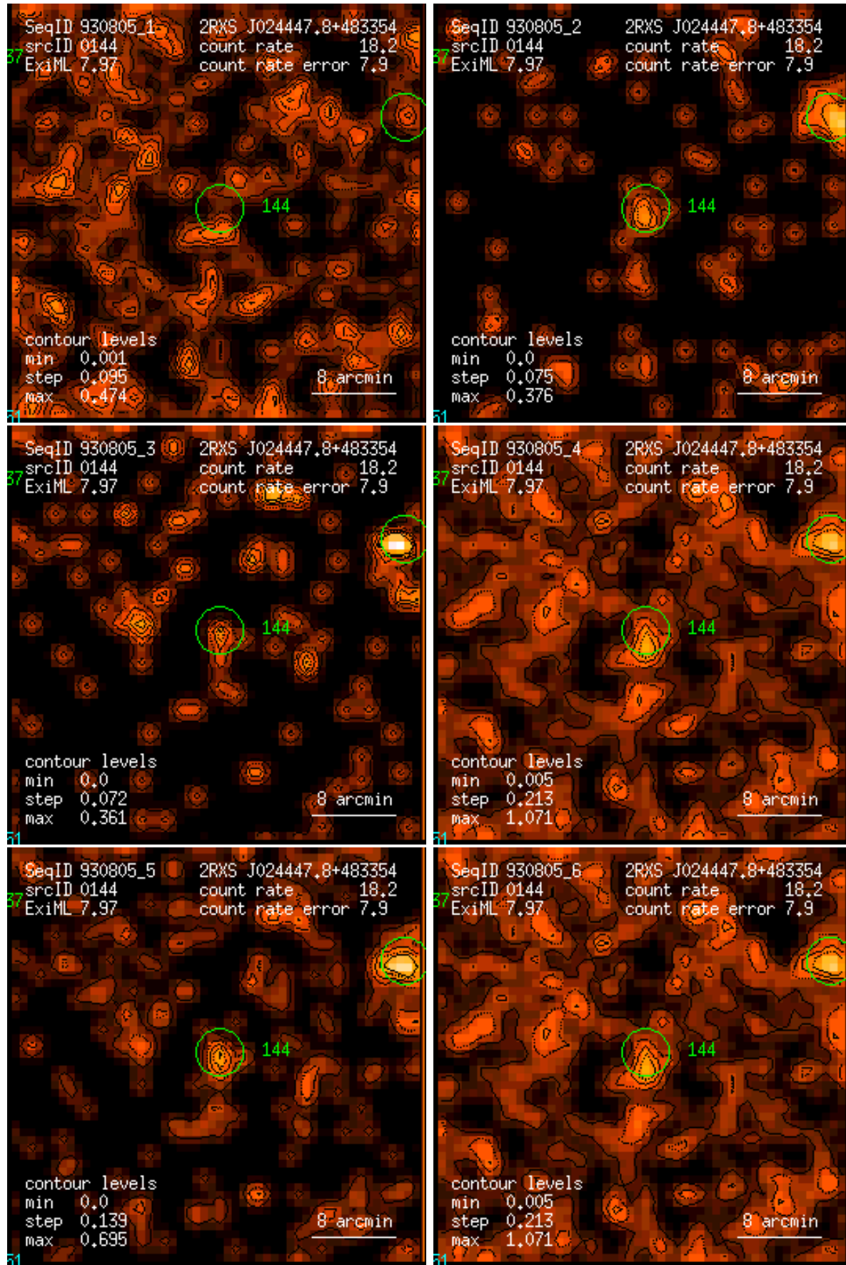
Figure 144: RASS 930805: detection 0144: band rate images, Gaussian filter: (1) PSPC channels 11 – 41, (2) 52 – 90, (3) 91 – 201, (4) 11 – 235, (5) 52 – 201, (6) 11 – 201. Broad band rates in counts/ks. Band rate contour levels in counts/ks/arcmin 2 .
