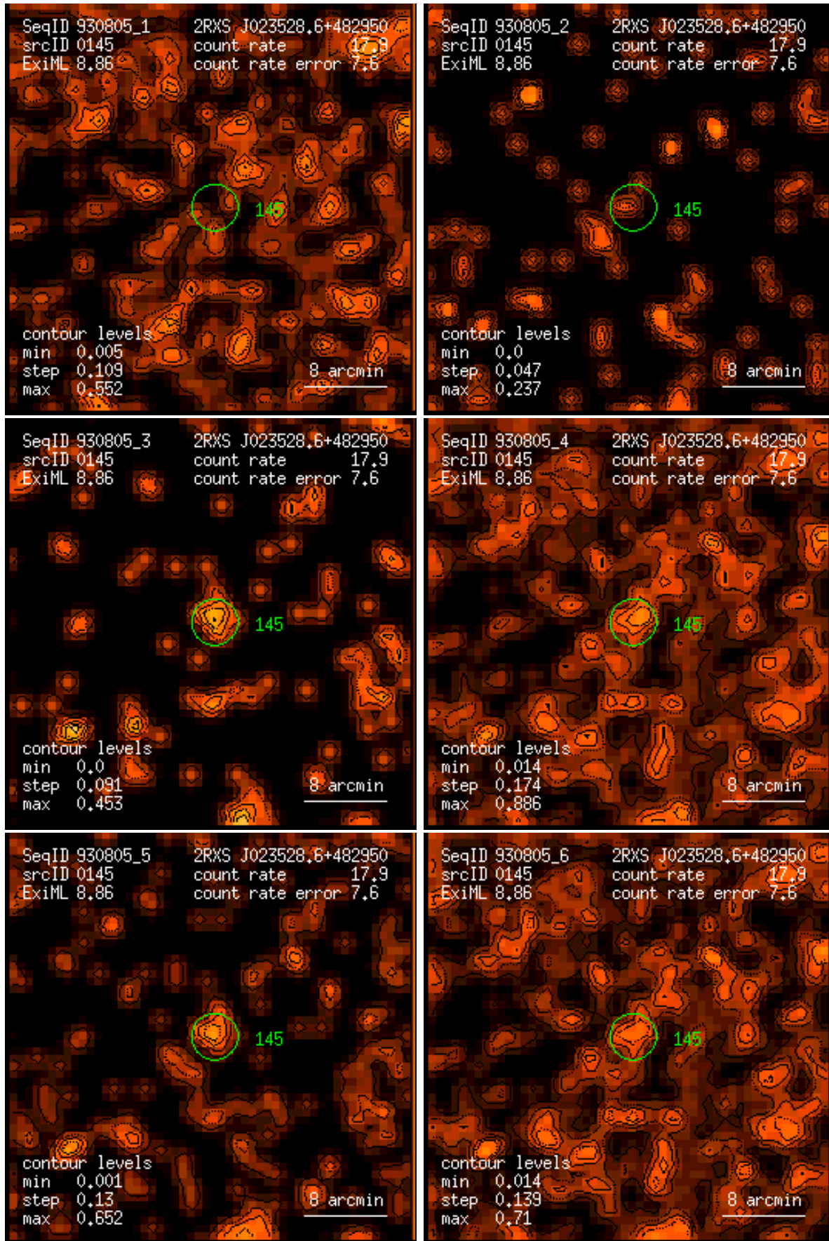
Figure 145: RASS 930805: detection 0145: band rate images, Gaussian filter: (1) PSPC channels 11 – 41, (2) 52 – 90, (3) 91 – 201, (4) 11 – 235, (5) 52 – 201, (6) 11 – 201. Broad band rates in counts/ks. Band rate contour levels in counts/ks/arcmin 2 .
