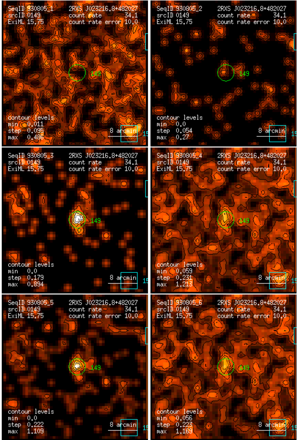
Figure 149: RASS 930805: detection 0149: band rate images, Gaussian filter: (1) PSPC channels 11 – 41, (2) 52 – 90, (3) 91 – 201, (4) 11 – 235, (5) 52 – 201, (6) 11 – 201. Broad band rates in counts/ks. Band rate contour levels in counts/ks/arcmin 2 .
