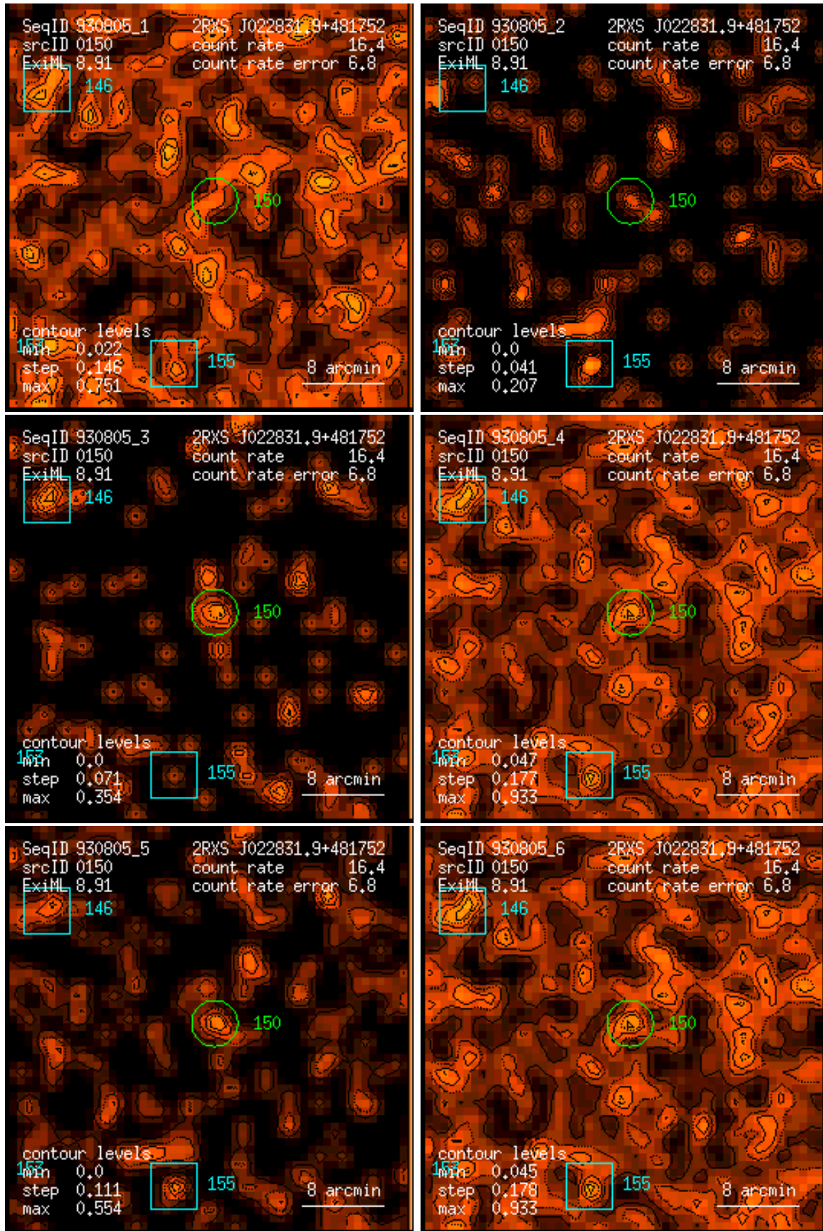
Figure 150: RASS 930805: detection 0150: band rate images, Gaussian filter: (1) PSPC channels 11 – 41, (2) 52 – 90, (3) 91 – 201, (4) 11 – 235, (5) 52 – 201, (6) 11 – 201. Broad band rates in counts/ks. Band rate contour levels in counts/ks/arcmin 2 .
