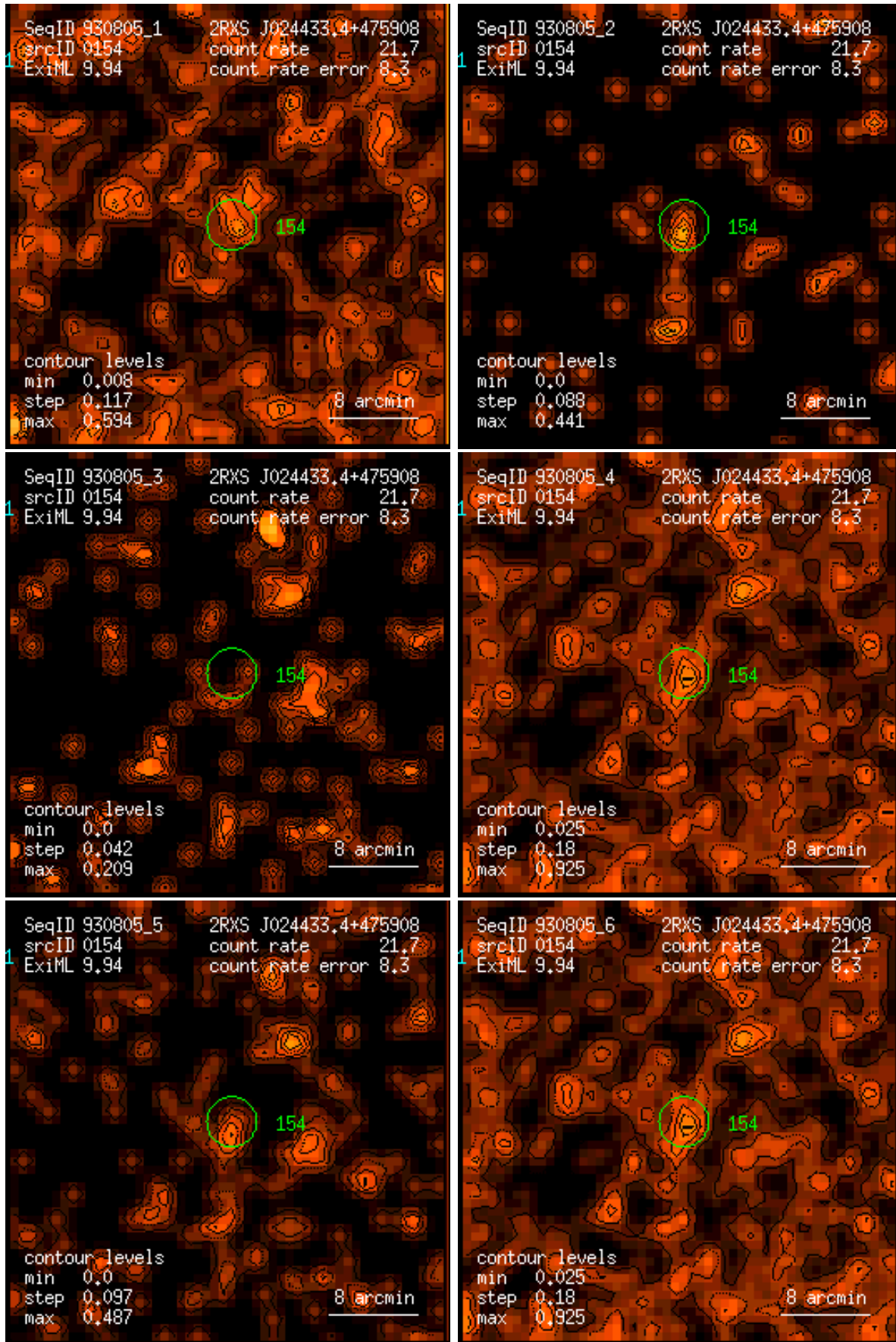
Figure 154: RASS 930805: detection 0154: band rate images, Gaussian filter: (1) PSPC channels 11 – 41, (2) 52 – 90, (3) 91 – 201, (4) 11 – 235, (5) 52 – 201, (6) 11 – 201. Broad band rates in counts/ks. Band rate contour levels in counts/ks/arcmin 2 .
