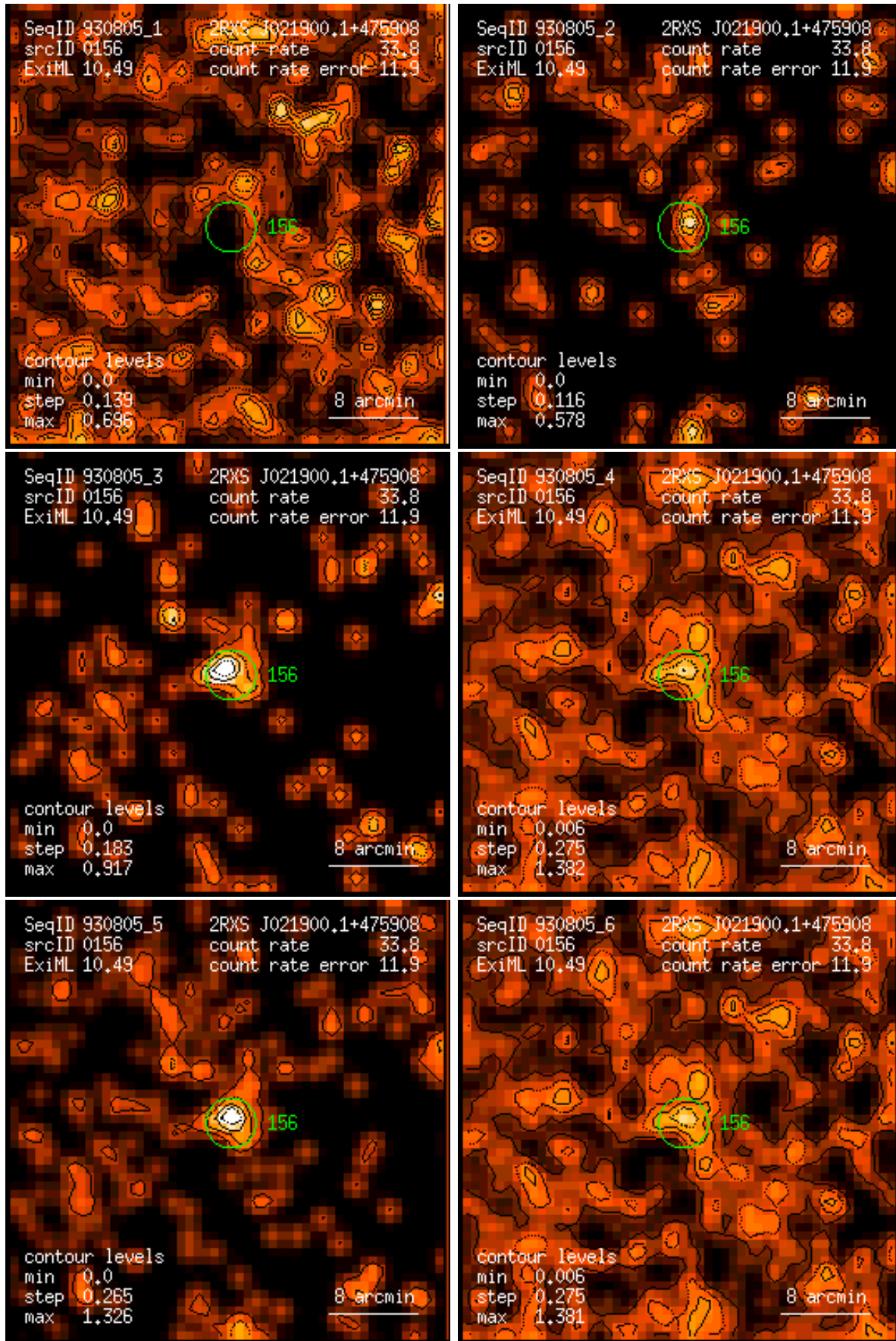
Figure 156: RASS 930805: detection 0156: band rate images, Gaussian filter: (1) PSPC channels 11 – 41, (2) 52 – 90, (3) 91 – 201, (4) 11 – 235, (5) 52 – 201, (6) 11 – 201. Broad band rates in counts/ks. Band rate contour levels in counts/ks/arcmin 2 .
