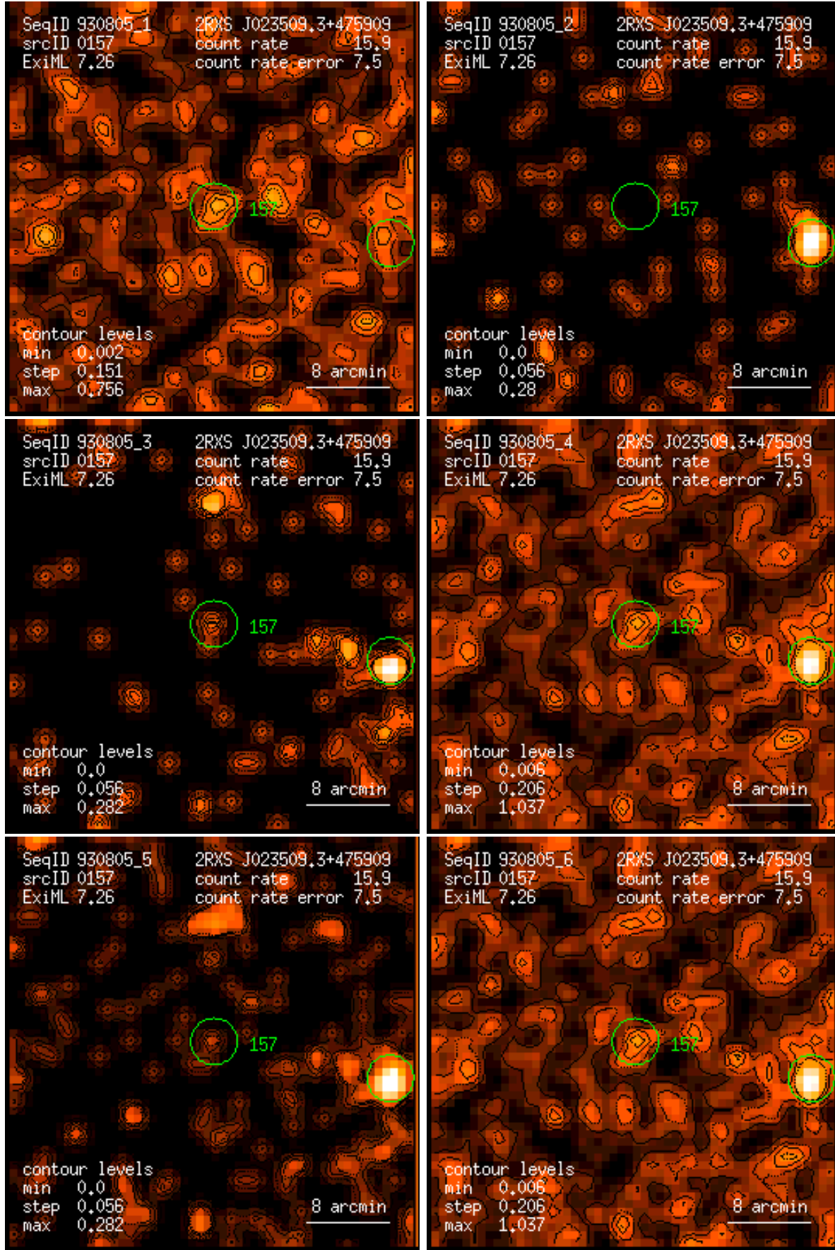
Figure 157: RASS 930805: detection 0157: band rate images, Gaussian filter: (1) PSPC channels 11 – 41, (2) 52 – 90, (3) 91 – 201, (4) 11 – 235, (5) 52 – 201, (6) 11 – 201. Broad band rates in counts/ks. Band rate contour levels in counts/ks/arcmin 2 .
