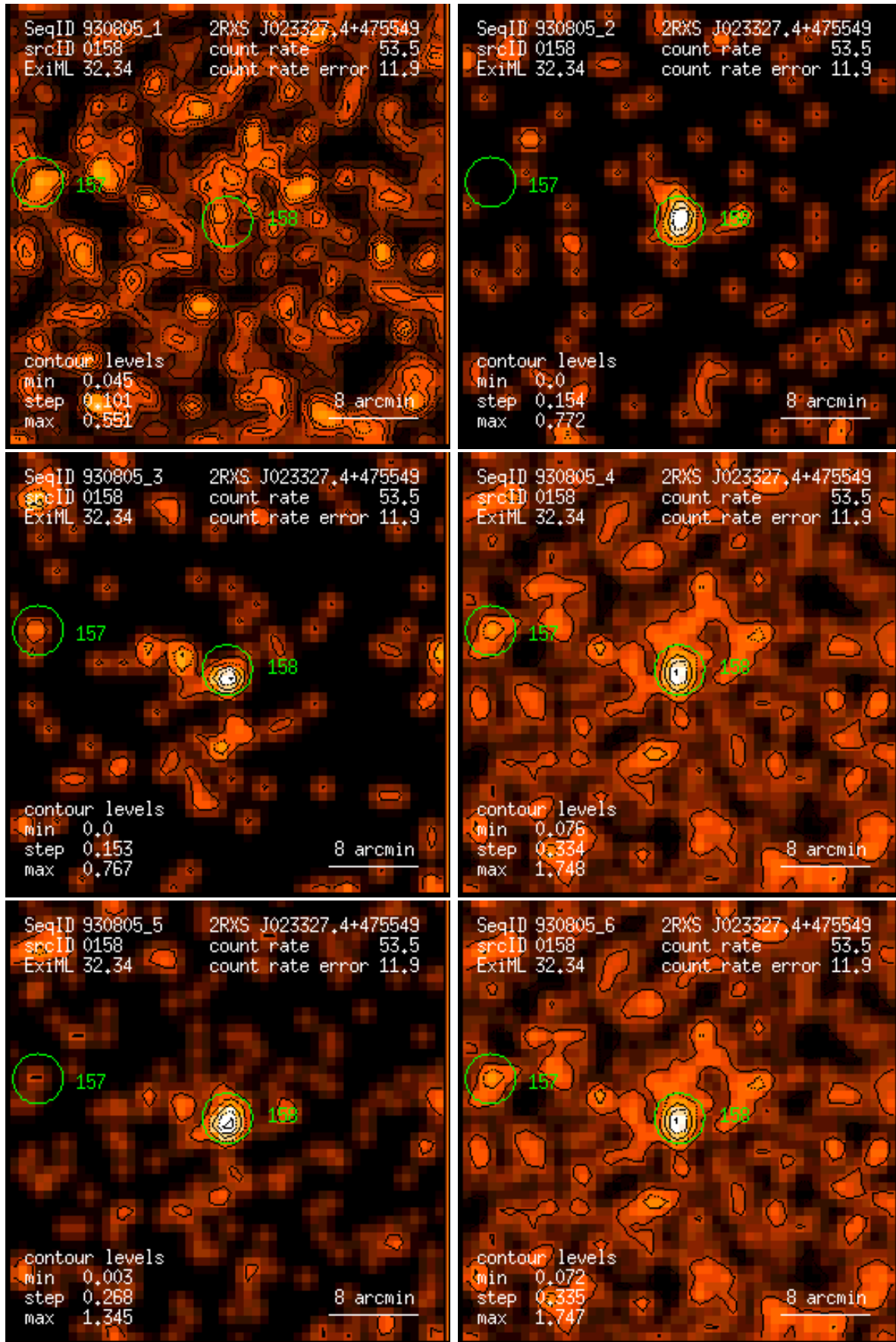
Figure 158: RASS 930805: detection 0158: band rate images, Gaussian filter: (1) PSPC channels 11 – 41, (2) 52 – 90, (3) 91 – 201, (4) 11 – 235, (5) 52 – 201, (6) 11 – 201. Broad band rates in counts/ks. Band rate contour levels in counts/ks/arcmin 2 .
