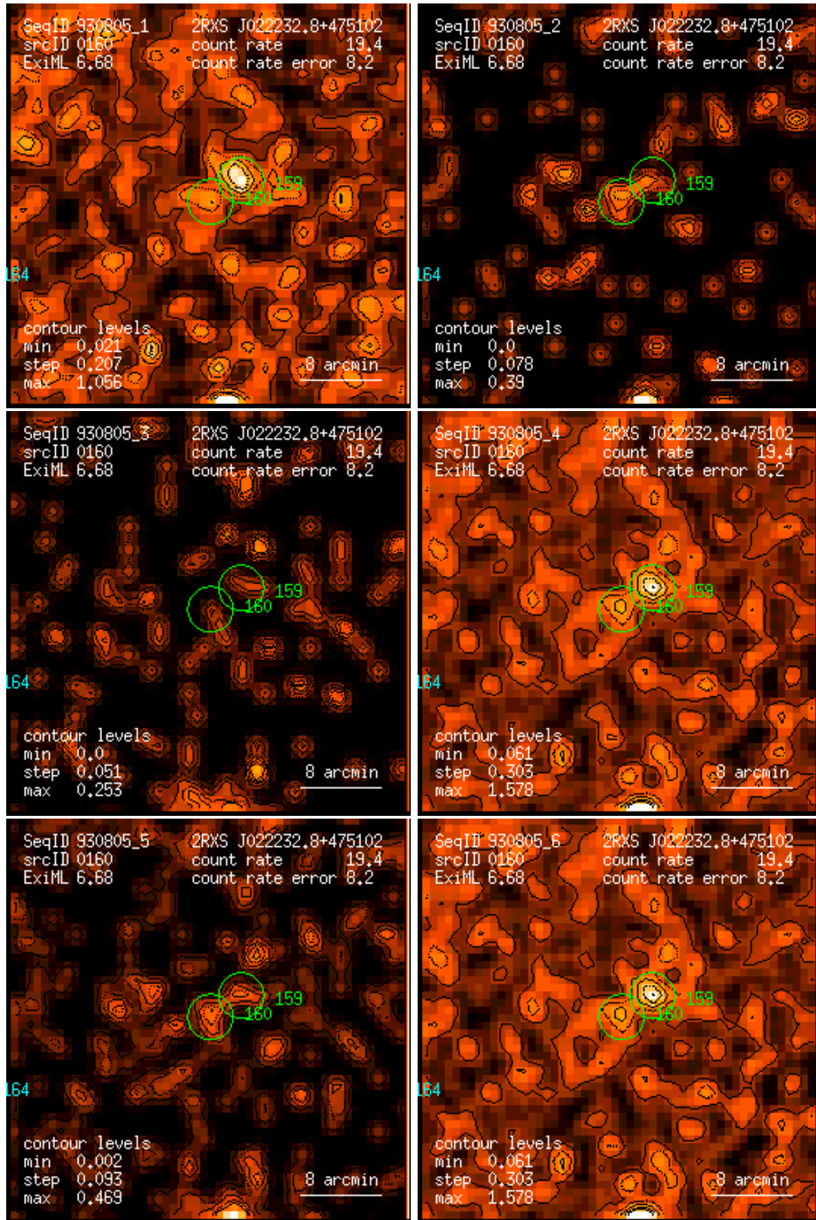
Figure 160: RASS 930805: detection 0160: band rate images, Gaussian filter: (1) PSPC channels 11 – 41, (2) 52 – 90, (3) 91 – 201, (4) 11 – 235, (5) 52 – 201, (6) 11 – 201. Broad band rates in counts/ks. Band rate contour levels in counts/ks/arcmin 2 .
