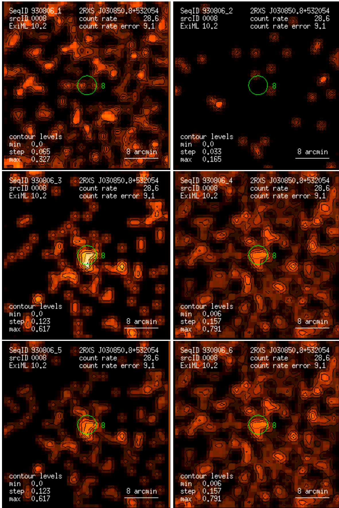
Figure 8: RASS 930806: detection 0008: band rate images, Gaussian filter: (1) PSPC channels 11 – 41, (2) 52 – 90, (3) 91 – 201, (4) 11 – 235, (5) 52 – 201, (6) 11 – 201. Broad band rates in counts/ks. Band rate contour levels in counts/ks/arcmin 2 .
