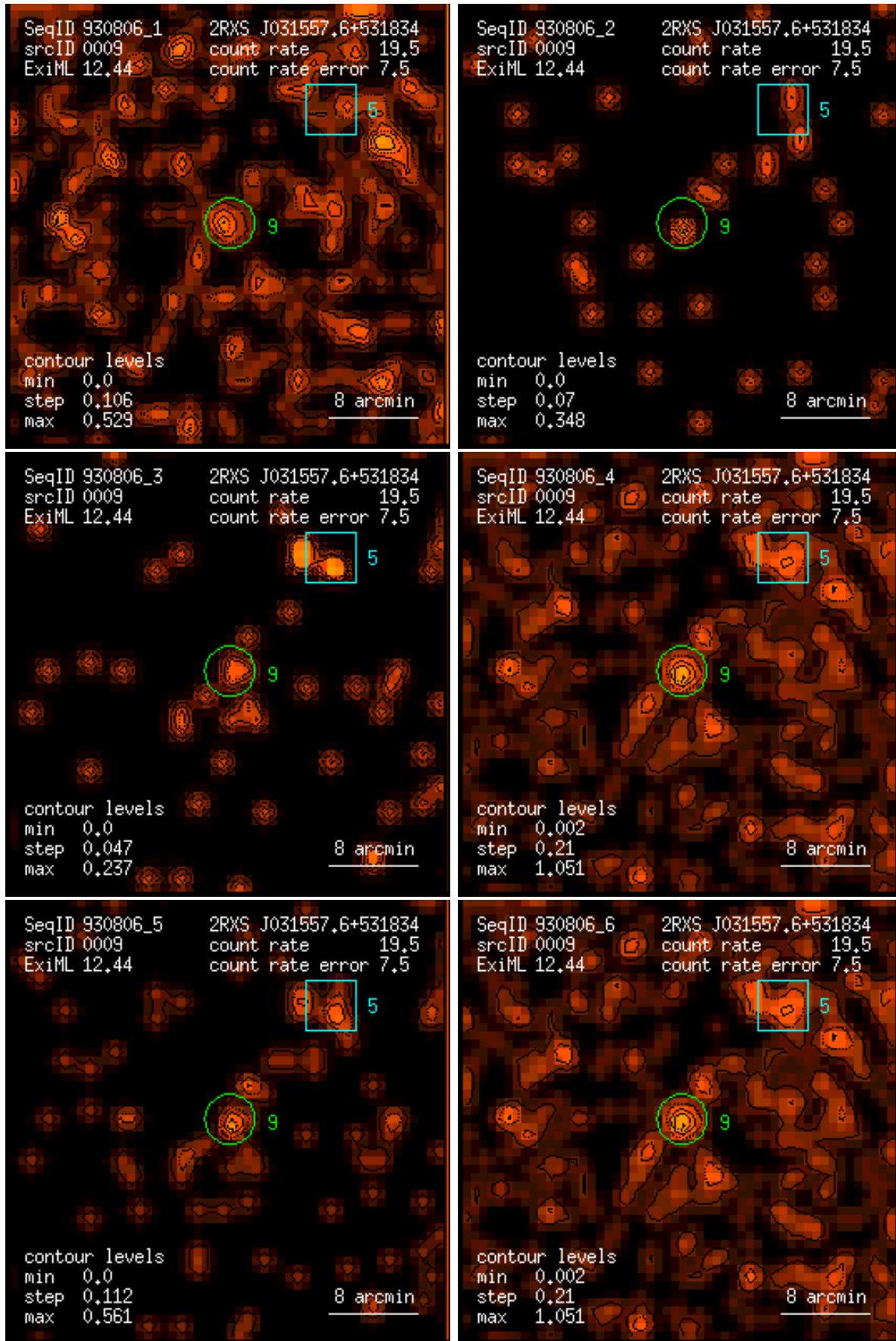
Figure 9: RASS 930806: detection 0009: band rate images, Gaussian filter: (1) PSPC channels 11 – 41, (2) 52 – 90, (3) 91 – 201, (4) 11 – 235, (5) 52 – 201, (6) 11 – 201. Broad band rates in counts/ks. Band rate contour levels in counts/ks/arcmin 2 .
