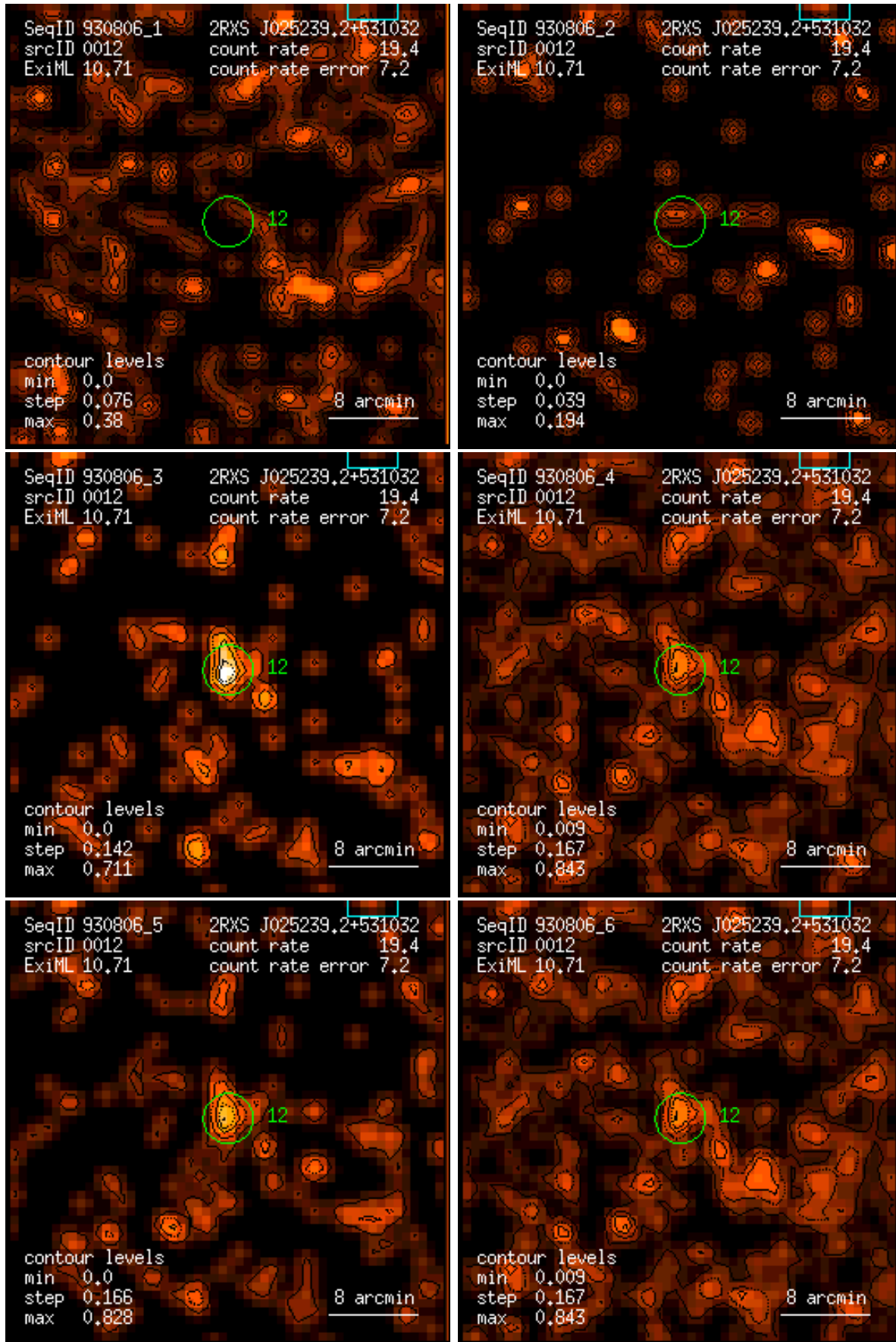
Figure 12: RASS 930806: detection 0012: band rate images, Gaussian filter: (1) PSPC channels 11 – 41, (2) 52 – 90, (3) 91 – 201, (4) 11 – 235, (5) 52 – 201, (6) 11 – 201. Broad band rates in counts/ks. Band rate contour levels in counts/ks/arcmin 2 .
