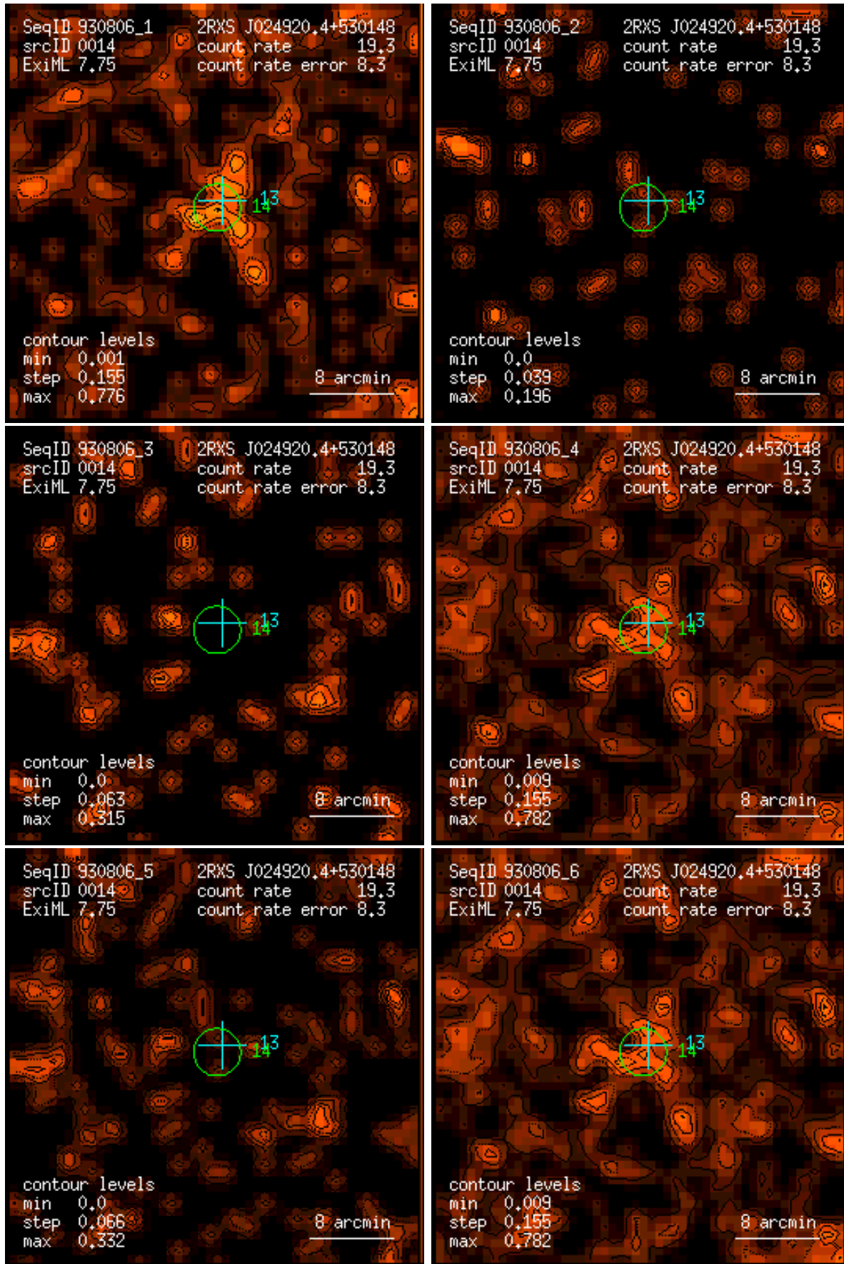
Figure 14: RASS 930806: detection 0014: band rate images, Gaussian filter: (1) PSPC channels 11 – 41, (2) 52 – 90, (3) 91 – 201, (4) 11 – 235, (5) 52 – 201, (6) 11 – 201. Broad band rates in counts/ks. Band rate contour levels in counts/ks/arcmin 2 .
