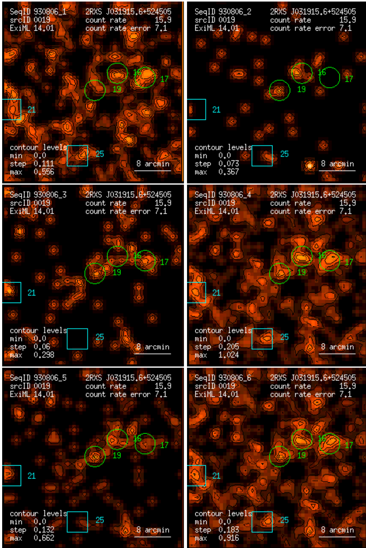
Figure 19: RASS 930806: detection 0019: band rate images, Gaussian filter: (1) PSPC channels 11 – 41, (2) 52 – 90, (3) 91 – 201, (4) 11 – 235, (5) 52 – 201, (6) 11 – 201. Broad band rates in counts/ks. Band rate contour levels in counts/ks/arcmin 2 .
