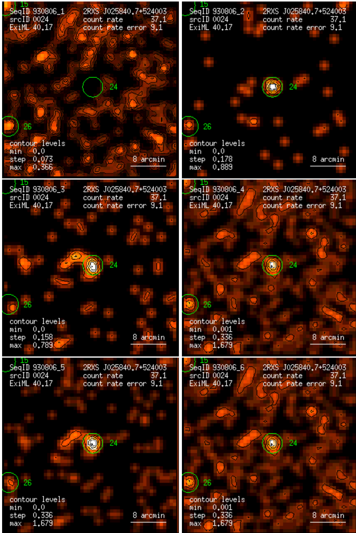
Figure 24: RASS 930806: detection 0024: band rate images, Gaussian filter: (1) PSPC channels 11 – 41, (2) 52 – 90, (3) 91 – 201, (4) 11 – 235, (5) 52 – 201, (6) 11 – 201. Broad band rates in counts/ks. Band rate contour levels in counts/ks/arcmin 2 .
