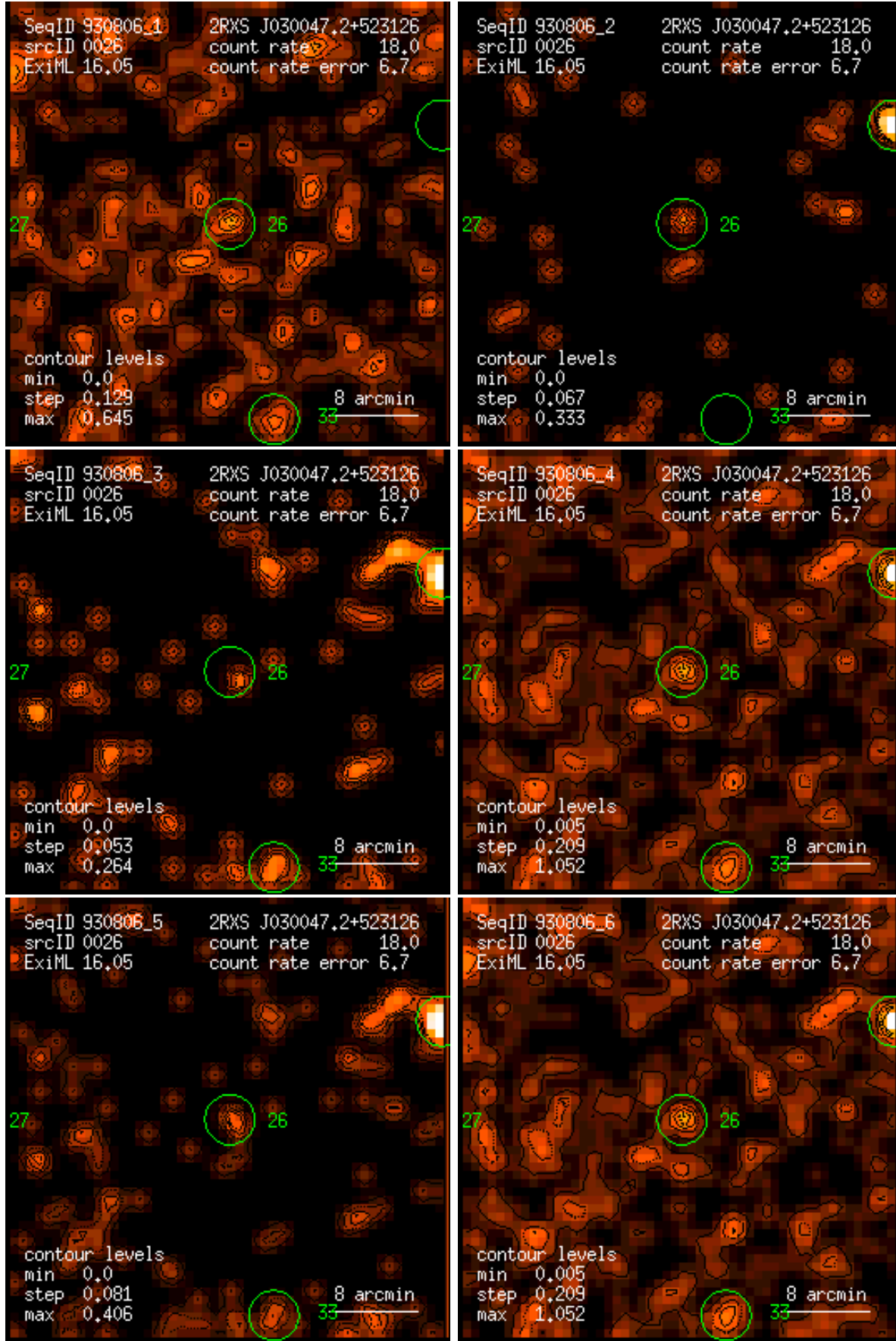
Figure 26: RASS 930806: detection 0026: band rate images, Gaussian filter: (1) PSPC channels 11 – 41, (2) 52 – 90, (3) 91 – 201, (4) 11 – 235, (5) 52 – 201, (6) 11 – 201. Broad band rates in counts/ks. Band rate contour levels in counts/ks/arcmin 2 .
