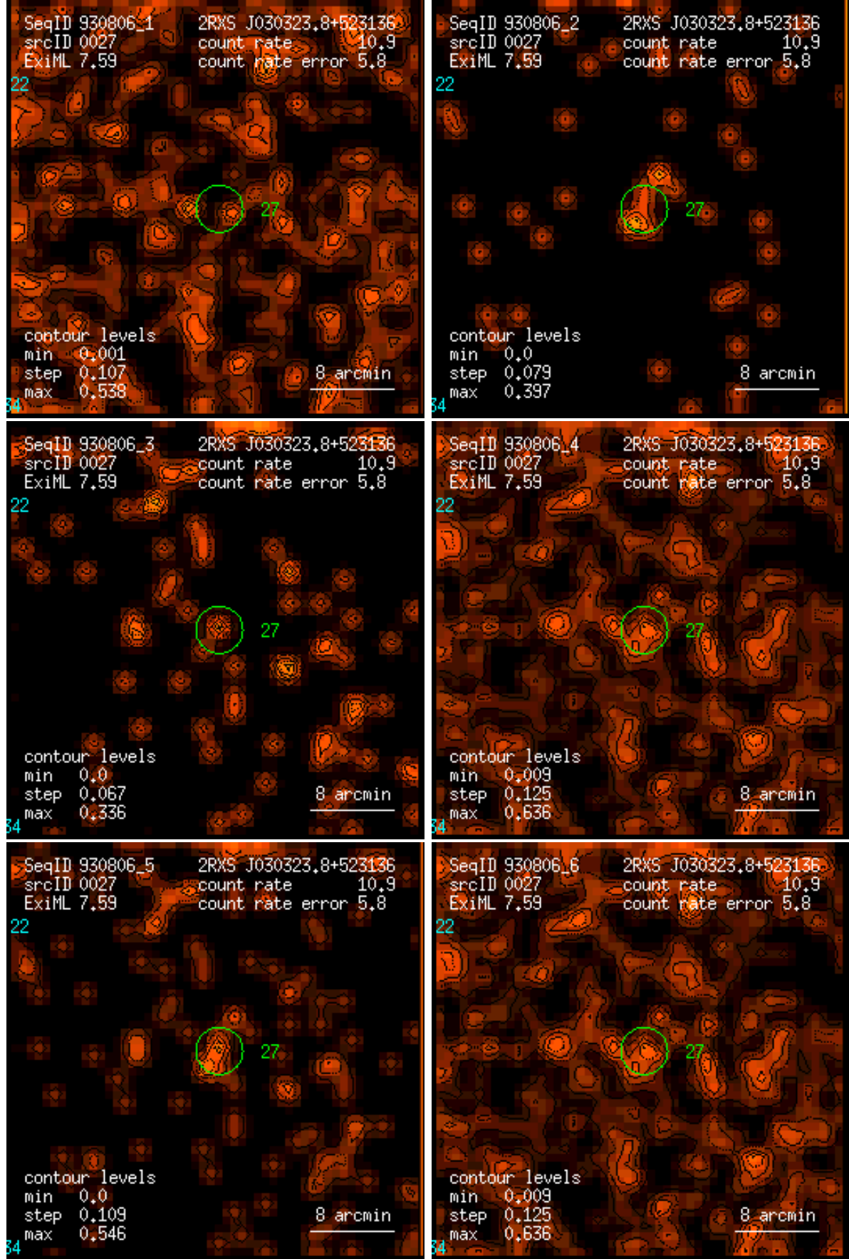
Figure 27: RASS 930806: detection 0027: band rate images, Gaussian filter: (1) PSPC channels 11 – 41, (2) 52 – 90, (3) 91 – 201, (4) 11 – 235, (5) 52 – 201, (6) 11 – 201. Broad band rates in counts/ks. Band rate contour levels in counts/ks/arcmin 2 .
