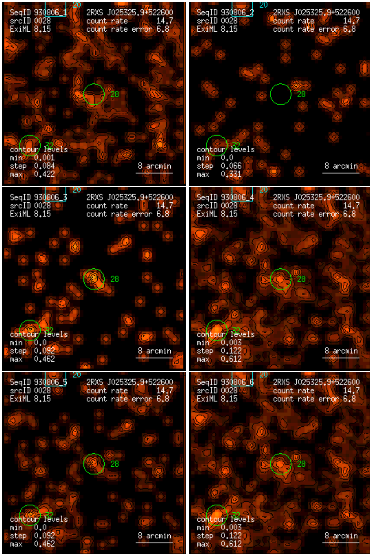
Figure 28: RASS 930806: detection 0028: band rate images, Gaussian filter: (1) PSPC channels 11 – 41, (2) 52 – 90, (3) 91 – 201, (4) 11 – 235, (5) 52 – 201, (6) 11 – 201. Broad band rates in counts/ks. Band rate contour levels in counts/ks/arcmin 2 .
