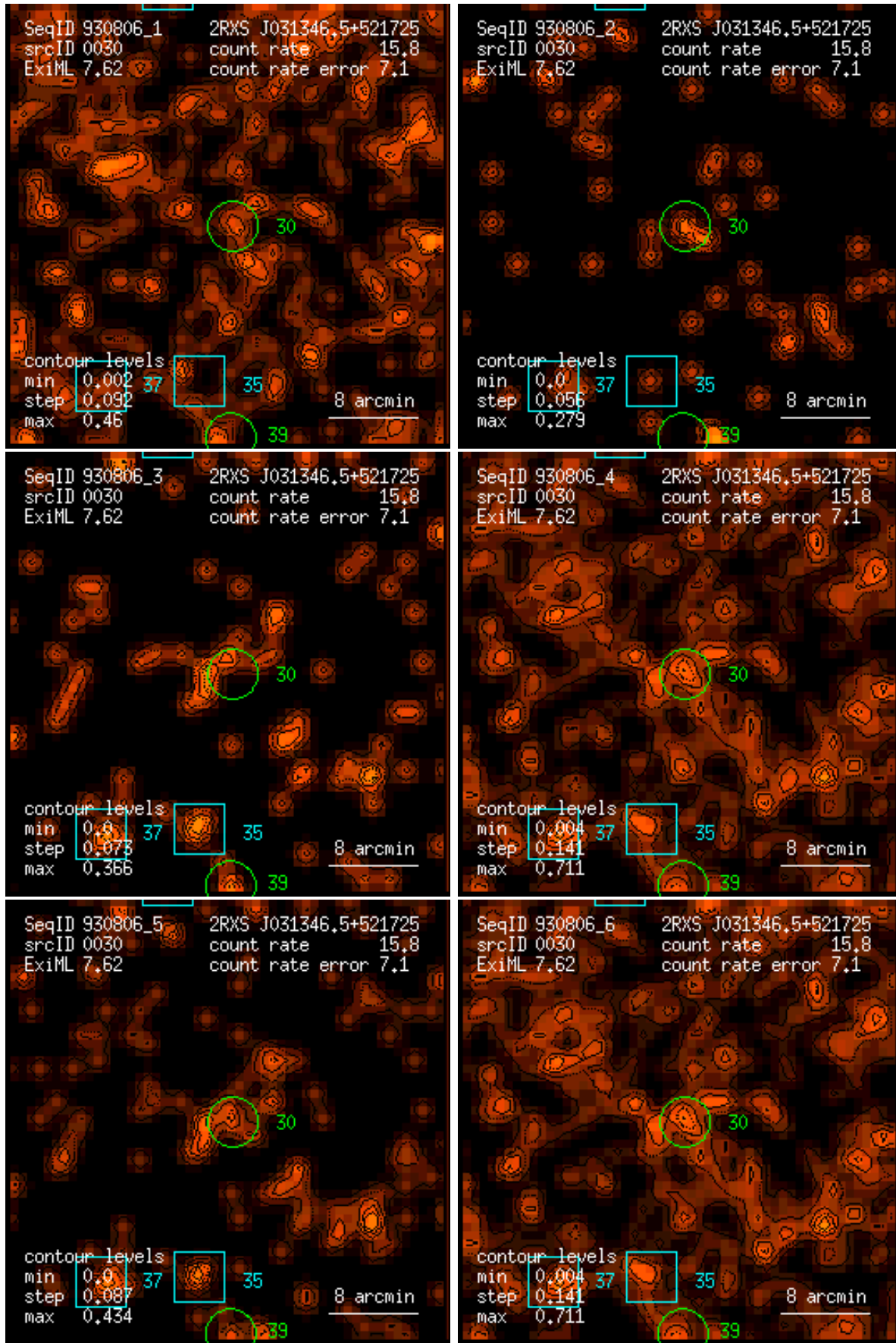
Figure 30: RASS 930806: detection 0030: band rate images, Gaussian filter: (1) PSPC channels 11 – 41, (2) 52 – 90, (3) 91 – 201, (4) 11 – 235, (5) 52 – 201, (6) 11 – 201. Broad band rates in counts/ks. Band rate contour levels in counts/ks/arcmin 2 .
