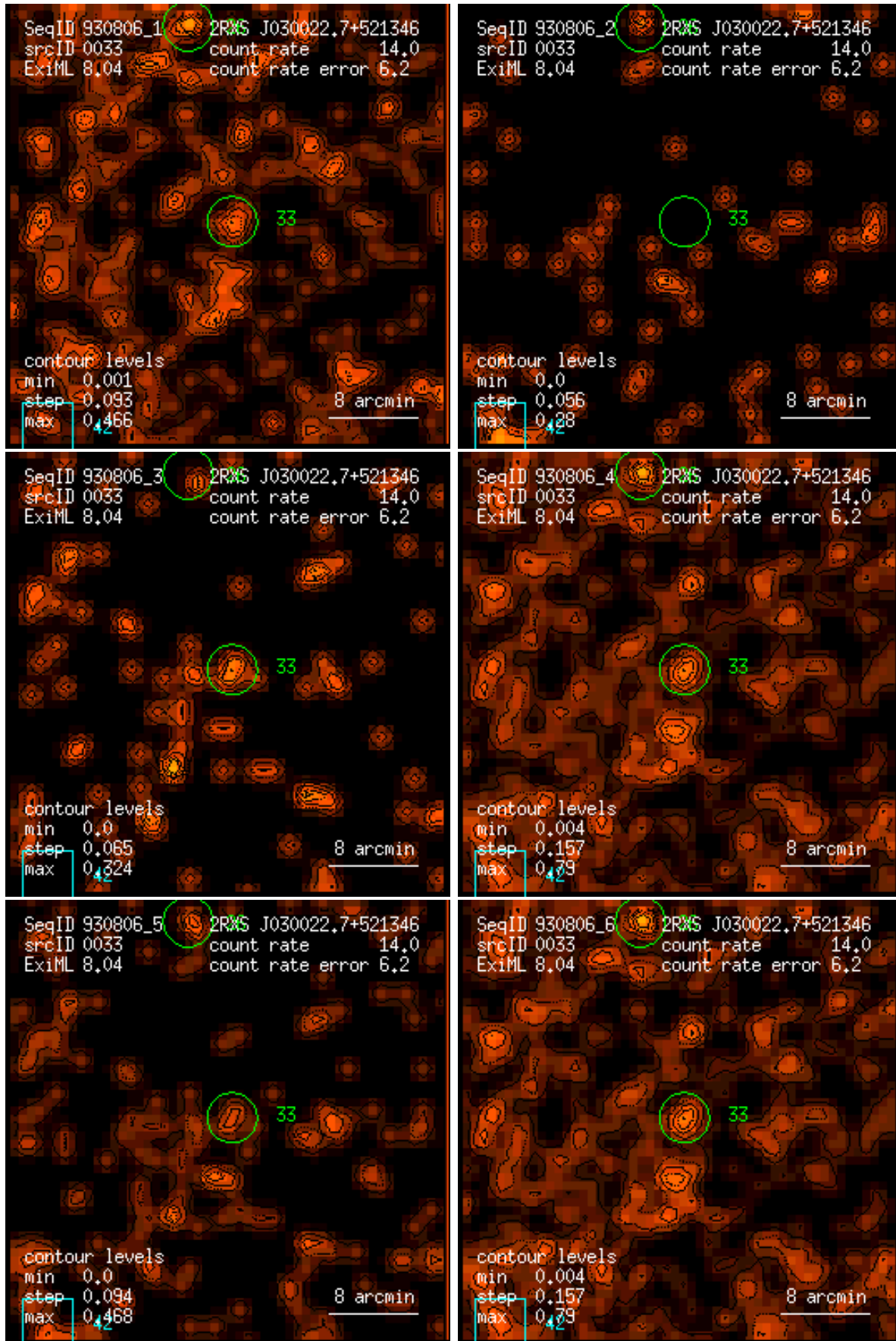
Figure 33: RASS 930806: detection 0033: band rate images, Gaussian filter: (1) PSPC channels 11 – 41, (2) 52 – 90, (3) 91 – 201, (4) 11 – 235, (5) 52 – 201, (6) 11 – 201. Broad band rates in counts/ks. Band rate contour levels in counts/ks/arcmin 2 .
