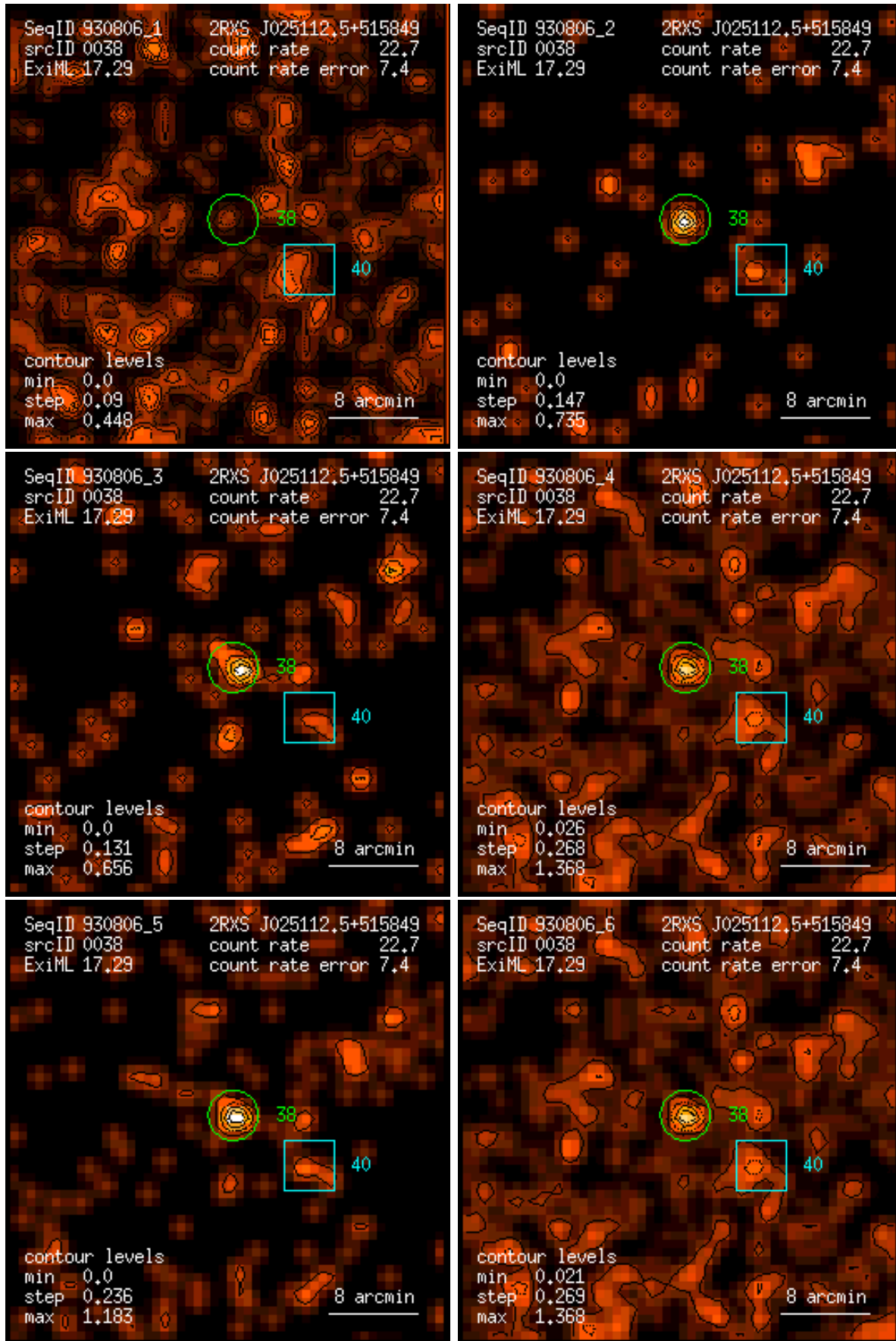
Figure 38: RASS 930806: detection 0038: band rate images, Gaussian filter: (1) PSPC channels 11 – 41, (2) 52 – 90, (3) 91 – 201, (4) 11 – 235, (5) 52 – 201, (6) 11 – 201. Broad band rates in counts/ks. Band rate contour levels in counts/ks/arcmin 2 .
