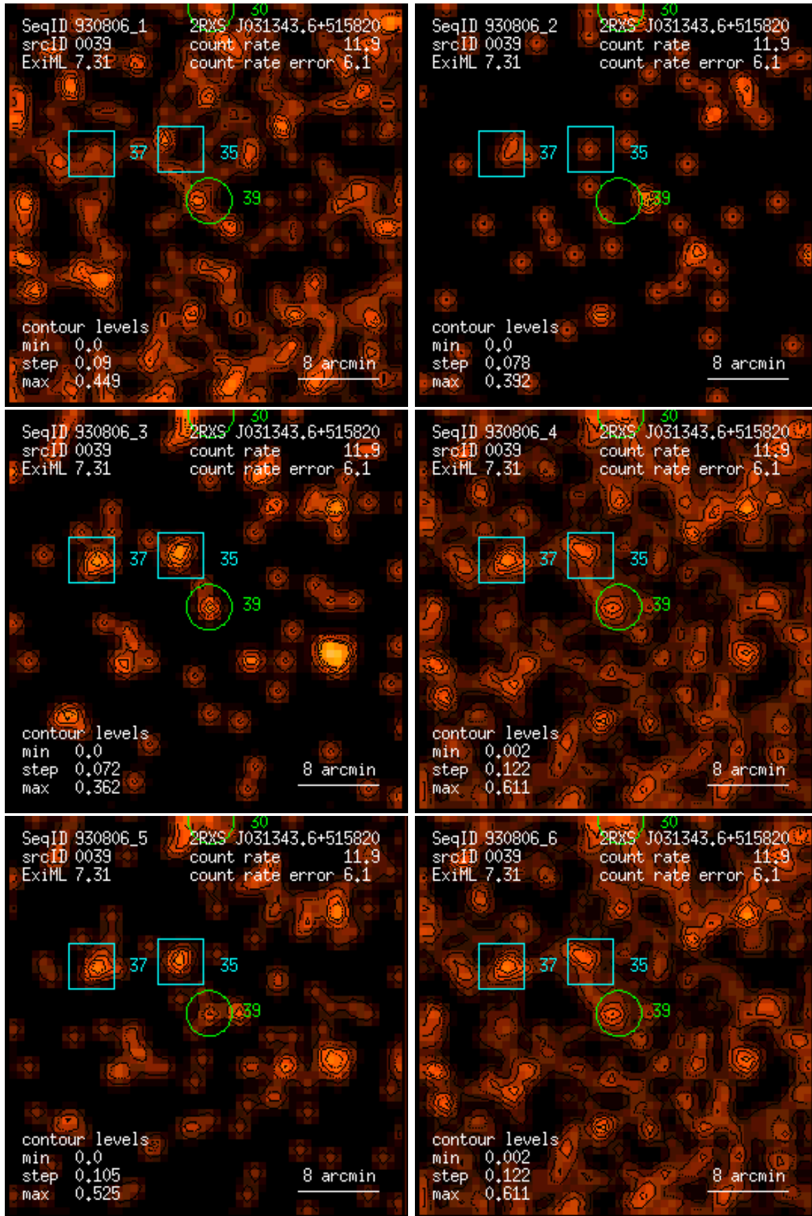
Figure 39: RASS 930806: detection 0039: band rate images, Gaussian filter: (1) PSPC channels 11 – 41, (2) 52 – 90, (3) 91 – 201, (4) 11 – 235, (5) 52 – 201, (6) 11 – 201. Broad band rates in counts/ks. Band rate contour levels in counts/ks/arcmin 2 .
