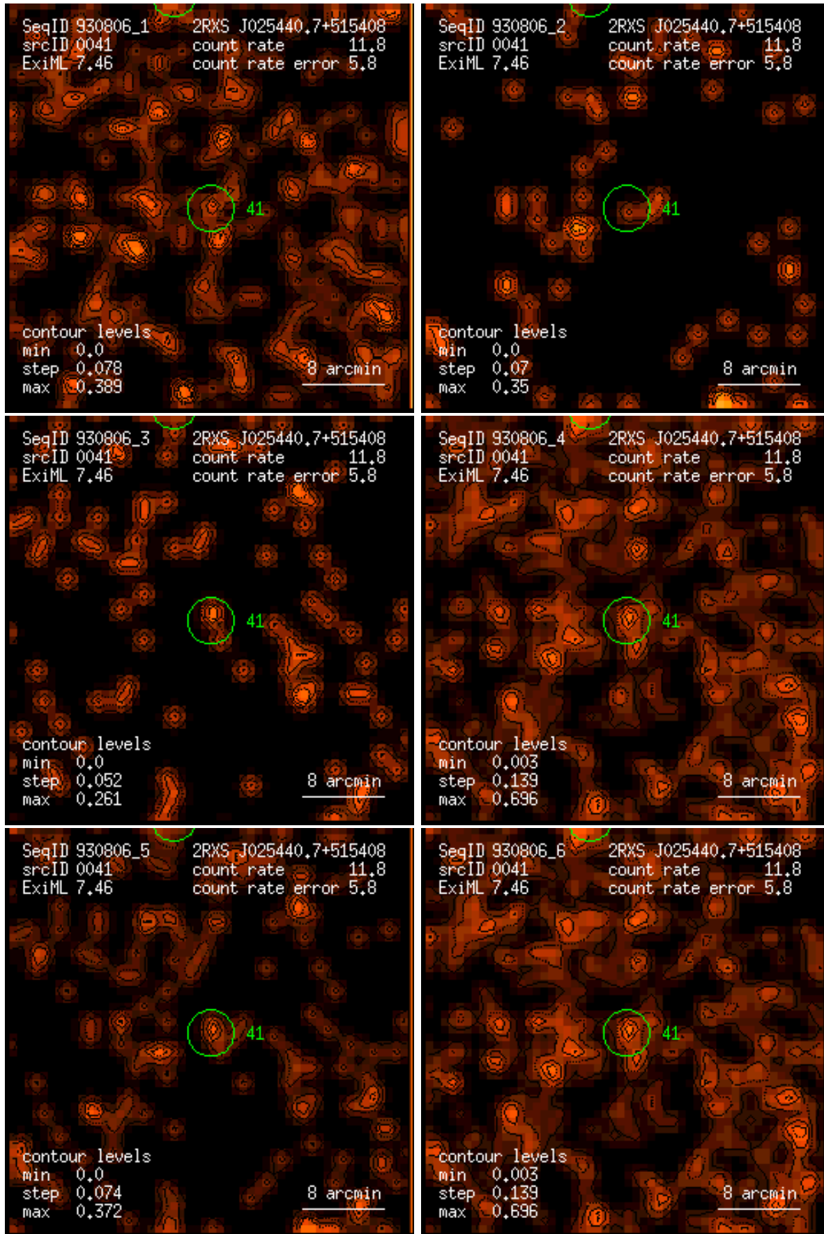
Figure 41: RASS 930806: detection 0041: band rate images, Gaussian filter: (1) PSPC channels 11 – 41, (2) 52 – 90, (3) 91 – 201, (4) 11 – 235, (5) 52 – 201, (6) 11 – 201. Broad band rates in counts/ks. Band rate contour levels in counts/ks/arcmin 2 .
