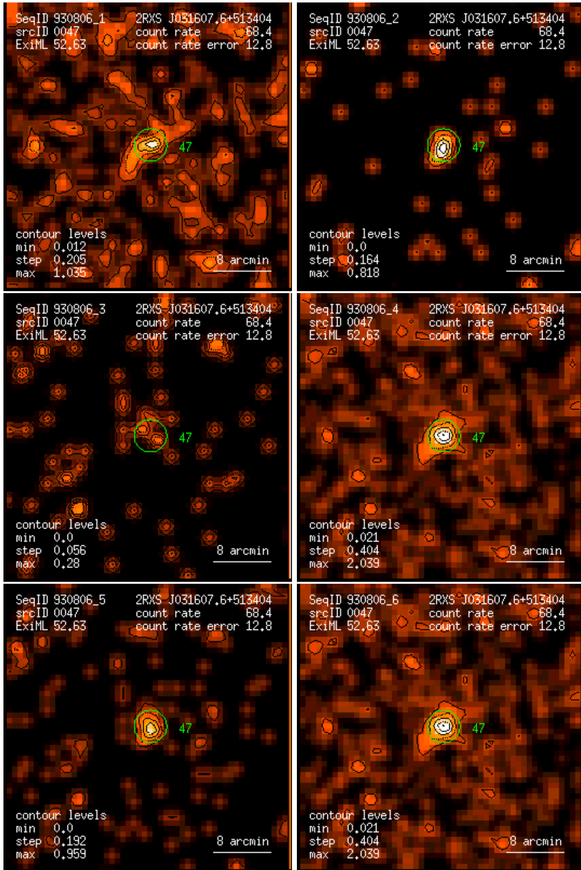
Figure 47: RASS 930806: detection 0047: band rate images, Gaussian filter: (1) PSPC channels 11 – 41, (2) 52 – 90, (3) 91 – 201, (4) 11 – 235, (5) 52 – 201, (6) 11 – 201. Broad band rates in counts/ks. Band rate contour levels in counts/ks/arcmin 2 .
