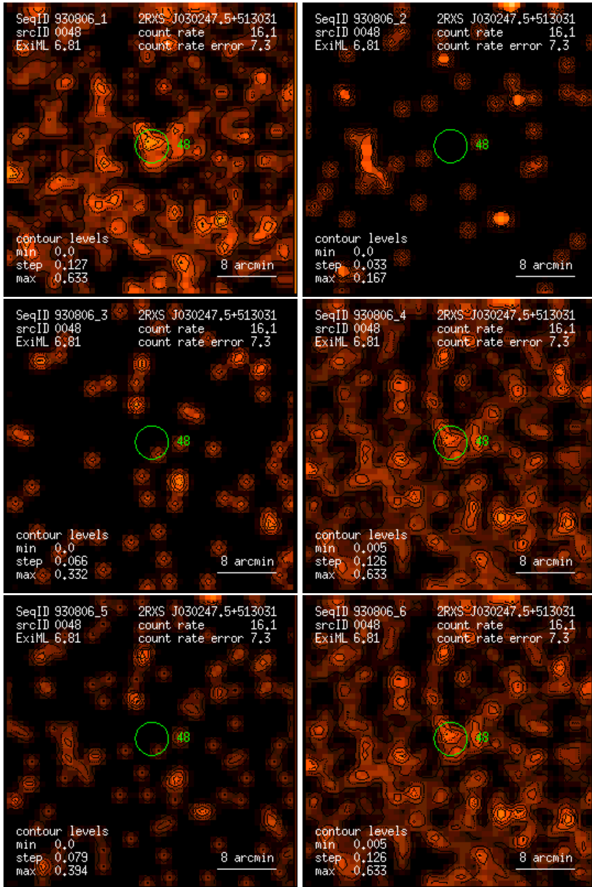
Figure 48: RASS 930806: detection 0048: band rate images, Gaussian filter: (1) PSPC channels 11 – 41, (2) 52 – 90, (3) 91 – 201, (4) 11 – 235, (5) 52 – 201, (6) 11 – 201. Broad band rates in counts/ks. Band rate contour levels in counts/ks/arcmin 2 .
