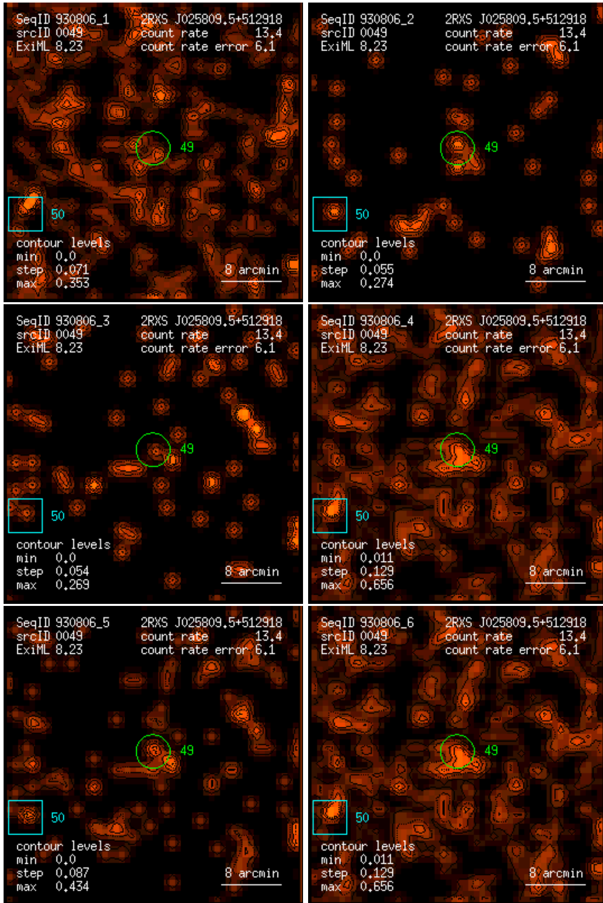
Figure 49: RASS 930806: detection 0049: band rate images, Gaussian filter: (1) PSPC channels 11 – 41, (2) 52 – 90, (3) 91 – 201, (4) 11 – 235, (5) 52 – 201, (6) 11 – 201. Broad band rates in counts/ks. Band rate contour levels in counts/ks/arcmin 2 .
