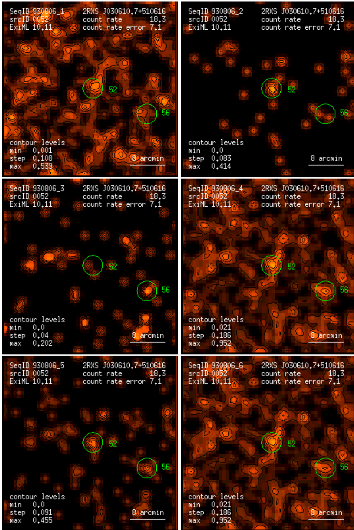
Figure 52: RASS 930806: detection 0052: band rate images, Gaussian filter: (1) PSPC channels 11 – 41, (2) 52 – 90, (3) 91 – 201, (4) 11 – 235, (5) 52 – 201, (6) 11 – 201. Broad band rates in counts/ks. Band rate contour levels in counts/ks/arcmin 2 .
