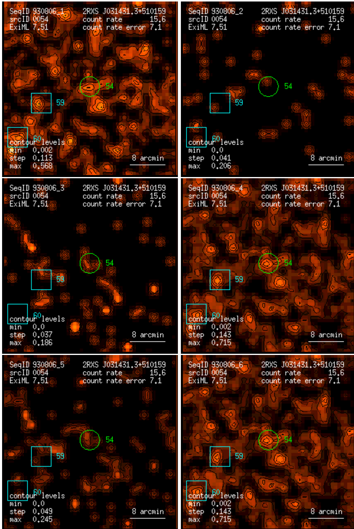
Figure 54: RASS 930806: detection 0054: band rate images, Gaussian filter: (1) PSPC channels 11 – 41, (2) 52 – 90, (3) 91 – 201, (4) 11 – 235, (5) 52 – 201, (6) 11 – 201. Broad band rates in counts/ks. Band rate contour levels in counts/ks/arcmin 2 .
