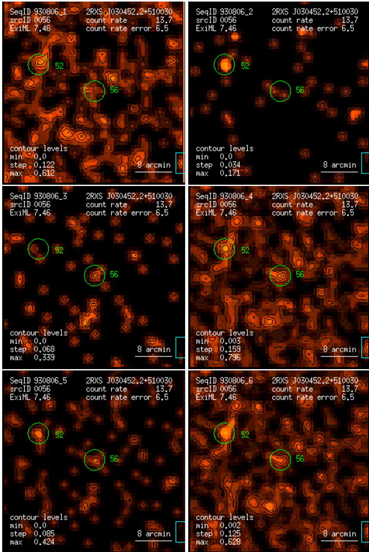
Figure 56: RASS 930806: detection 0056: band rate images, Gaussian filter: (1) PSPC channels 11 – 41, (2) 52 – 90, (3) 91 – 201, (4) 11 – 235, (5) 52 – 201, (6) 11 – 201. Broad band rates in counts/ks. Band rate contour levels in counts/ks/arcmin 2 .
