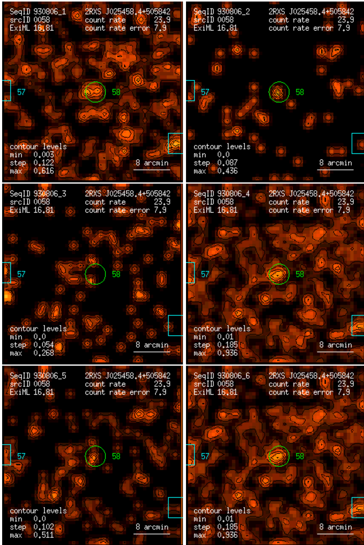
Figure 58: RASS 930806: detection 0058: band rate images, Gaussian filter: (1) PSPC channels 11 – 41, (2) 52 – 90, (3) 91 – 201, (4) 11 – 235, (5) 52 – 201, (6) 11 – 201. Broad band rates in counts/ks. Band rate contour levels in counts/ks/arcmin 2 .
