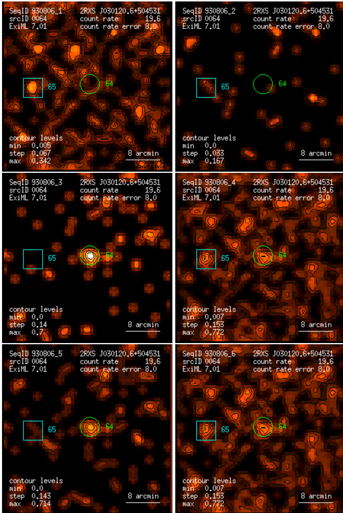
Figure 64: RASS 930806: detection 0064: band rate images, Gaussian filter: (1) PSPC channels 11 – 41, (2) 52 – 90, (3) 91 – 201, (4) 11 – 235, (5) 52 – 201, (6) 11 – 201. Broad band rates in counts/ks. Band rate contour levels in counts/ks/arcmin 2 .
