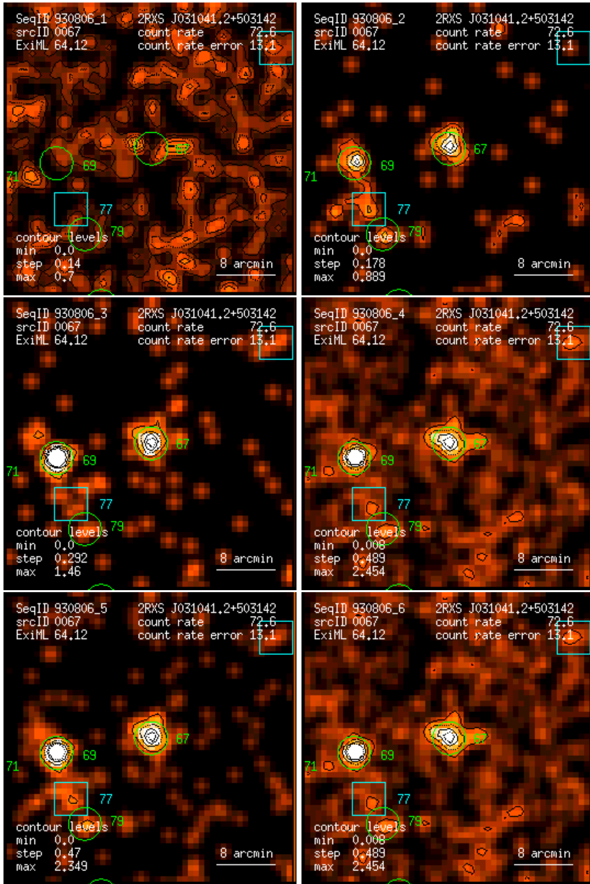
Figure 67: RASS 930806: detection 0067: band rate images, Gaussian filter: (1) PSPC channels 11 – 41, (2) 52 – 90, (3) 91 – 201, (4) 11 – 235, (5) 52 – 201, (6) 11 – 201. Broad band rates in counts/ks. Band rate contour levels in counts/ks/arcmin 2 .
