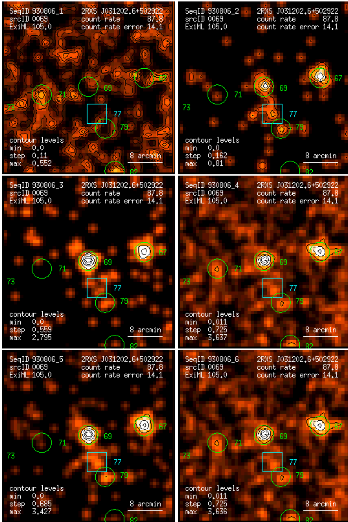
Figure 69: RASS 930806: detection 0069: band rate images, Gaussian filter: (1) PSPC channels 11 – 41, (2) 52 – 90, (3) 91 – 201, (4) 11 – 235, (5) 52 – 201, (6) 11 – 201. Broad band rates in counts/ks. Band rate contour levels in counts/ks/arcmin 2 .
