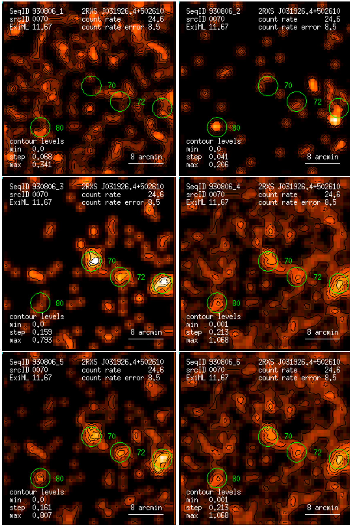
Figure 70: RASS 930806: detection 0070: band rate images, Gaussian filter: (1) PSPC channels 11 – 41, (2) 52 – 90, (3) 91 – 201, (4) 11 – 235, (5) 52 – 201, (6) 11 – 201. Broad band rates in counts/ks. Band rate contour levels in counts/ks/arcmin 2 .
