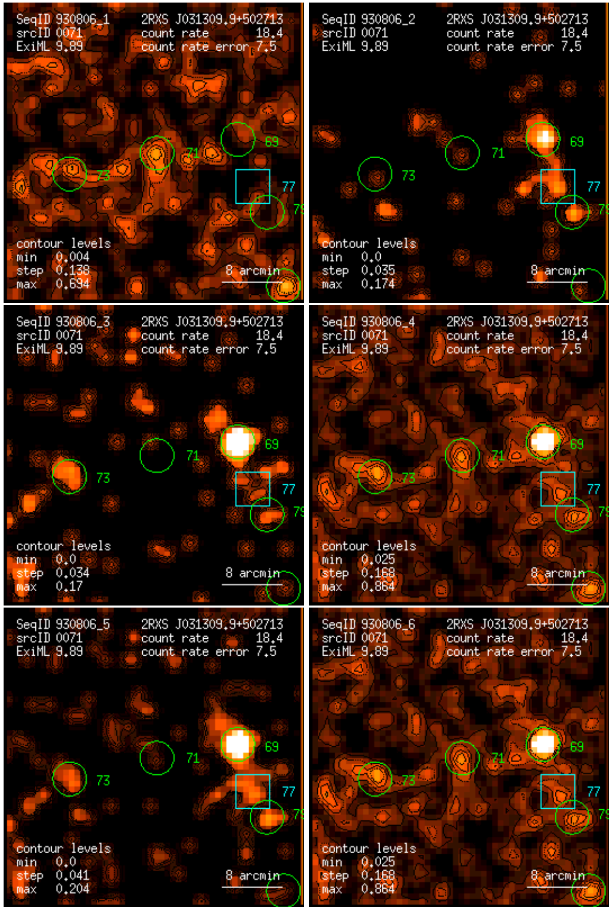
Figure 71: RASS 930806: detection 0071: band rate images, Gaussian filter: (1) PSPC channels 11 – 41, (2) 52 – 90, (3) 91 – 201, (4) 11 – 235, (5) 52 – 201, (6) 11 – 201. Broad band rates in counts/ks. Band rate contour levels in counts/ks/arcmin 2 .
