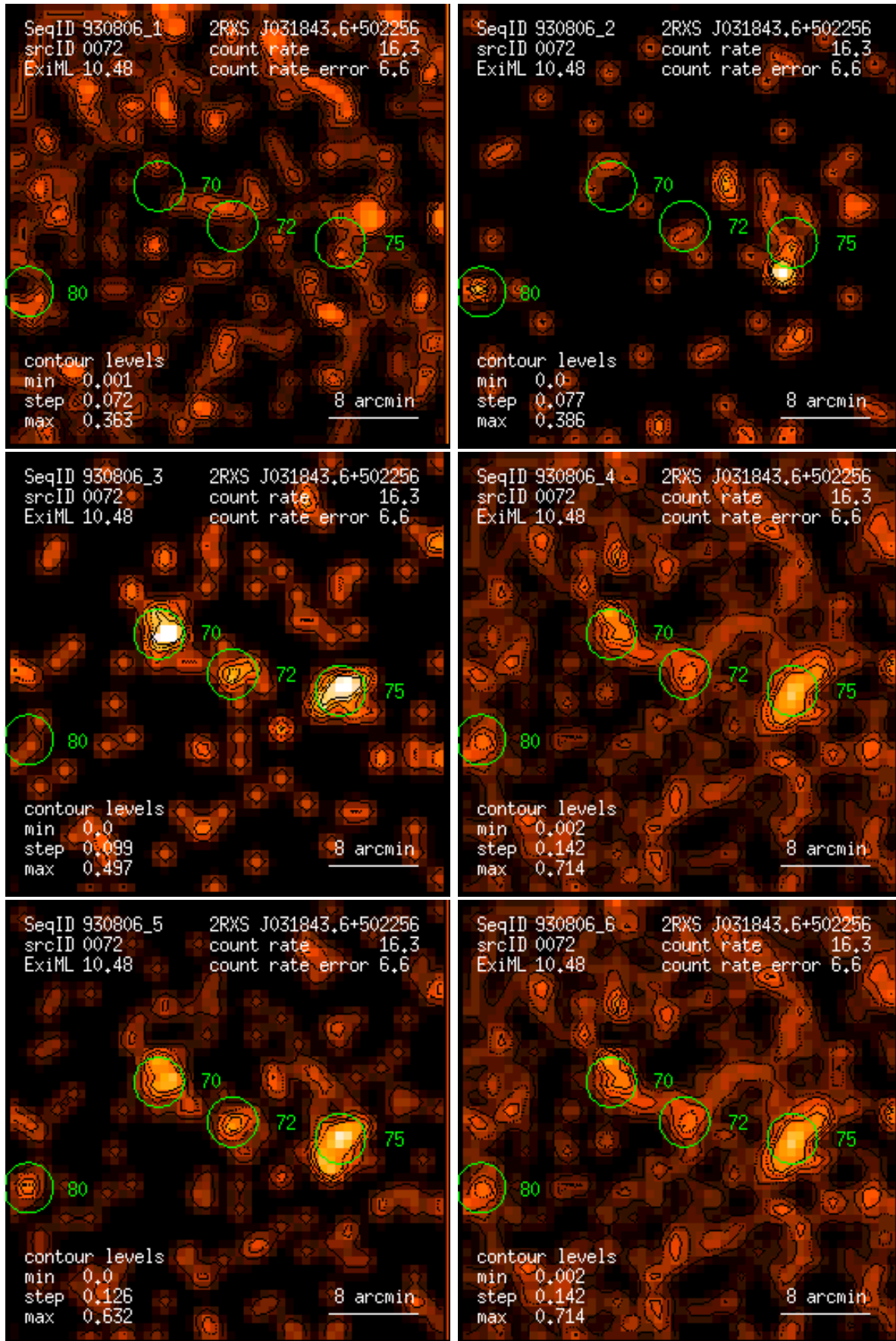
Figure 72: RASS 930806: detection 0072: band rate images, Gaussian filter: (1) PSPC channels 11 – 41, (2) 52 – 90, (3) 91 – 201, (4) 11 – 235, (5) 52 – 201, (6) 11 – 201. Broad band rates in counts/ks. Band rate contour levels in counts/ks/arcmin 2 .
