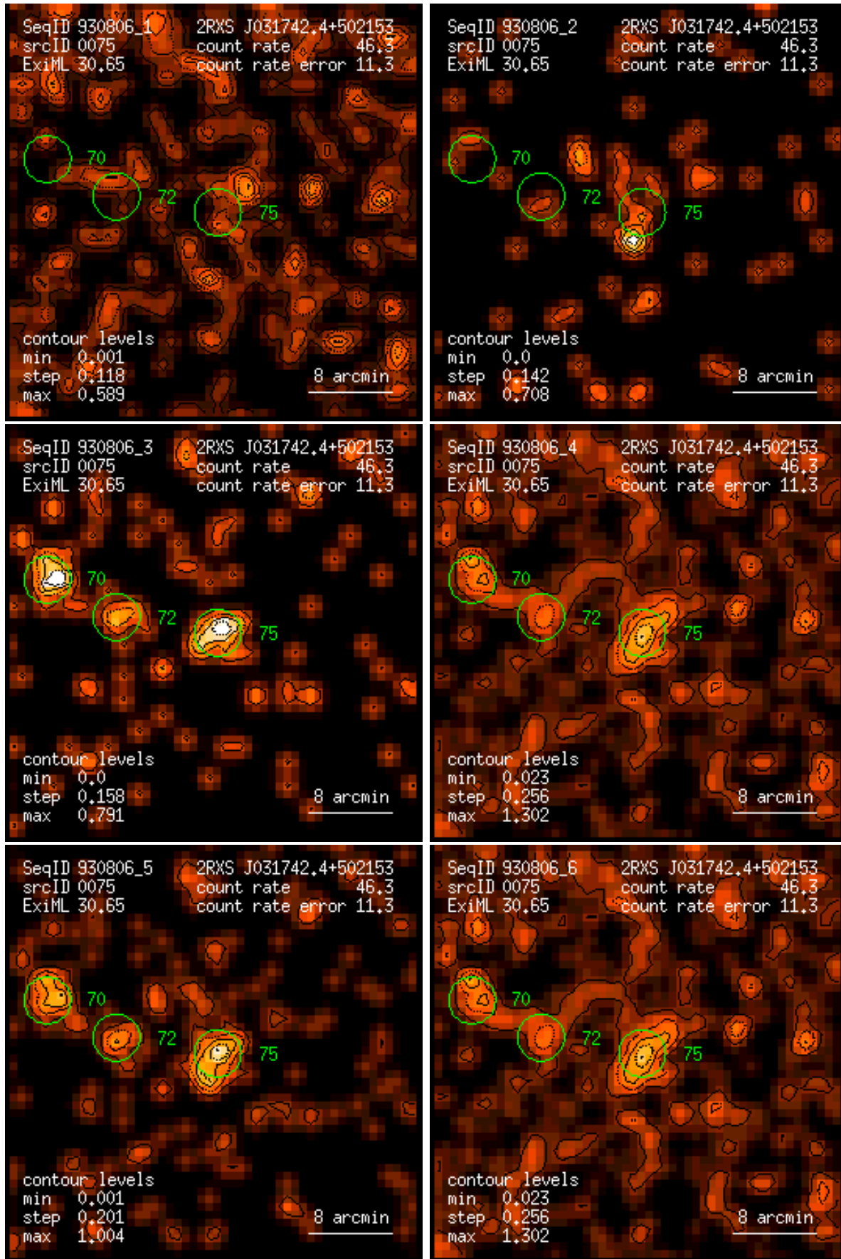
Figure 75: RASS 930806: detection 0075: band rate images, Gaussian filter: (1) PSPC channels 11 – 41, (2) 52 – 90, (3) 91 – 201, (4) 11 – 235, (5) 52 – 201, (6) 11 – 201. Broad band rates in counts/ks. Band rate contour levels in counts/ks/arcmin 2 .
