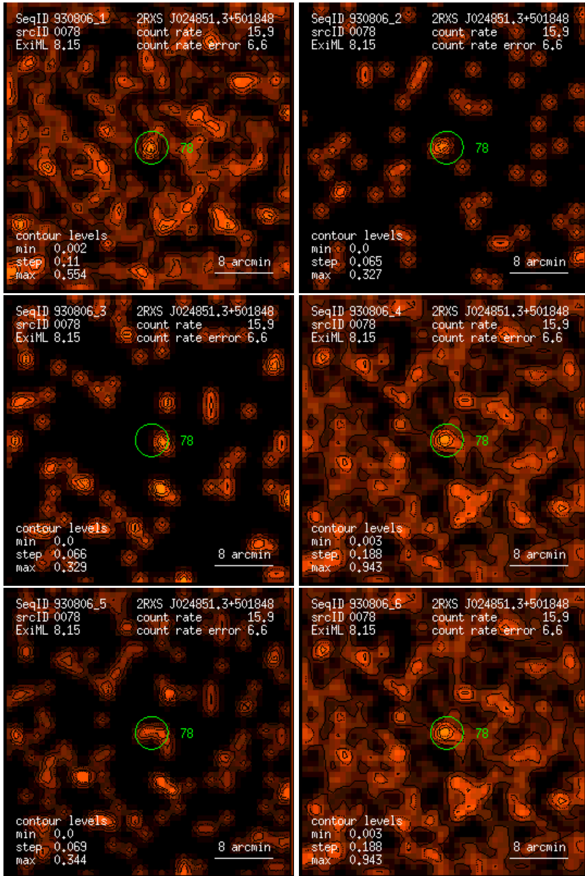
Figure 78: RASS 930806: detection 0078: band rate images, Gaussian filter: (1) PSPC channels 11 – 41, (2) 52 – 90, (3) 91 – 201, (4) 11 – 235, (5) 52 – 201, (6) 11 – 201. Broad band rates in counts/ks. Band rate contour levels in counts/ks/arcmin 2 .
