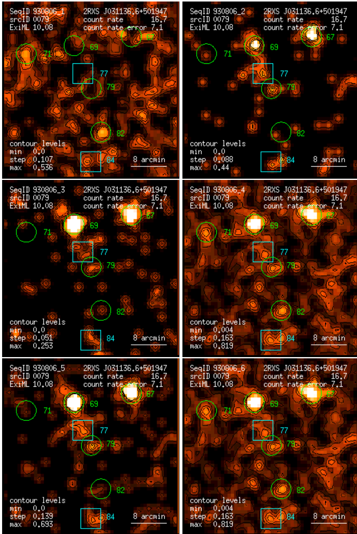
Figure 79: RASS 930806: detection 0079: band rate images, Gaussian filter: (1) PSPC channels 11 – 41, (2) 52 – 90, (3) 91 – 201, (4) 11 – 235, (5) 52 – 201, (6) 11 – 201. Broad band rates in counts/ks. Band rate contour levels in counts/ks/arcmin 2 .
