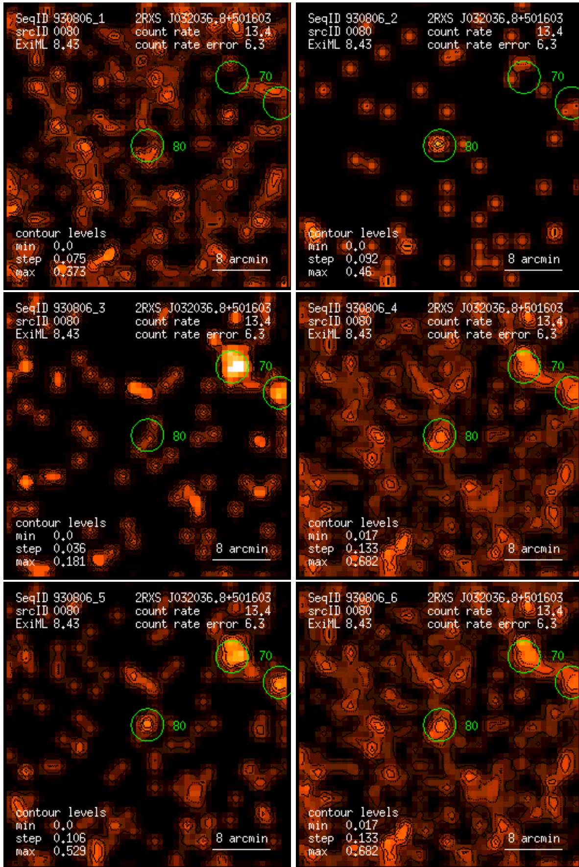
Figure 80: RASS 930806: detection 0080: band rate images, Gaussian filter: (1) PSPC channels 11 – 41, (2) 52 – 90, (3) 91 – 201, (4) 11 – 235, (5) 52 – 201, (6) 11 – 201. Broad band rates in counts/ks. Band rate contour levels in counts/ks/arcmin 2 .
