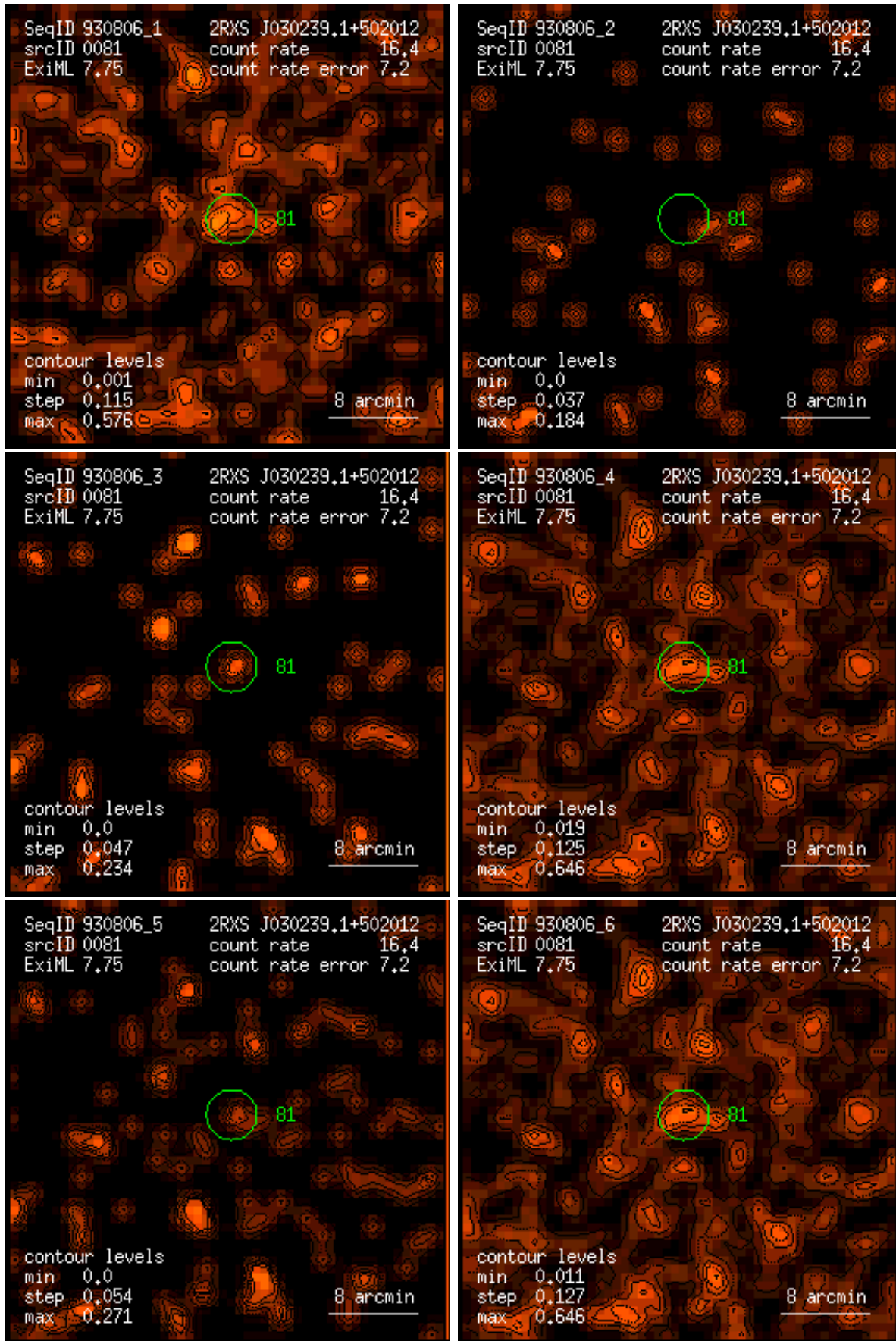
Figure 81: RASS 930806: detection 0081: band rate images, Gaussian filter: (1) PSPC channels 11 – 41, (2) 52 – 90, (3) 91 – 201, (4) 11 – 235, (5) 52 – 201, (6) 11 – 201. Broad band rates in counts/ks. Band rate contour levels in counts/ks/arcmin 2 .
