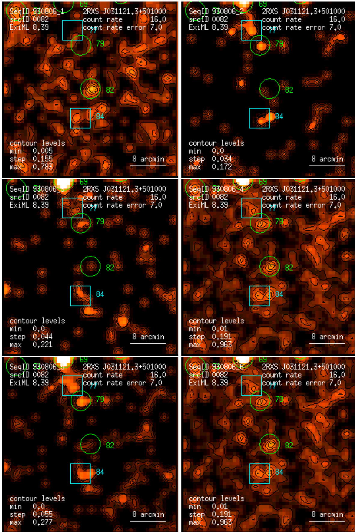
Figure 82: RASS 930806: detection 0082: band rate images, Gaussian filter: (1) PSPC channels 11 – 41, (2) 52 – 90, (3) 91 – 201, (4) 11 – 235, (5) 52 – 201, (6) 11 – 201. Broad band rates in counts/ks. Band rate contour levels in counts/ks/arcmin 2 .
