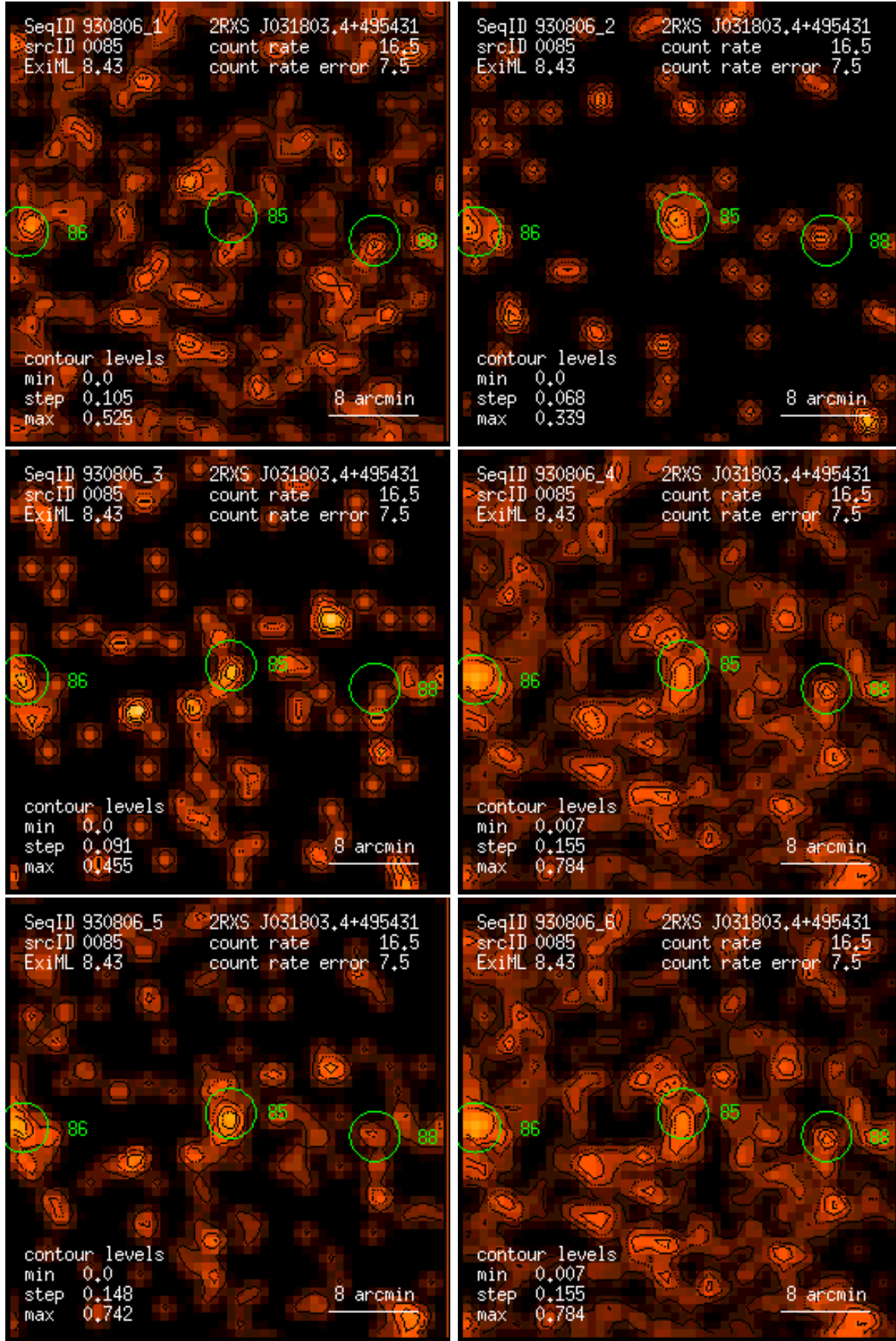
Figure 85: RASS 930806: detection 0085: band rate images, Gaussian filter: (1) PSPC channels 11 – 41, (2) 52 – 90, (3) 91 – 201, (4) 11 – 235, (5) 52 – 201, (6) 11 – 201. Broad band rates in counts/ks. Band rate contour levels in counts/ks/arcmin 2 .
