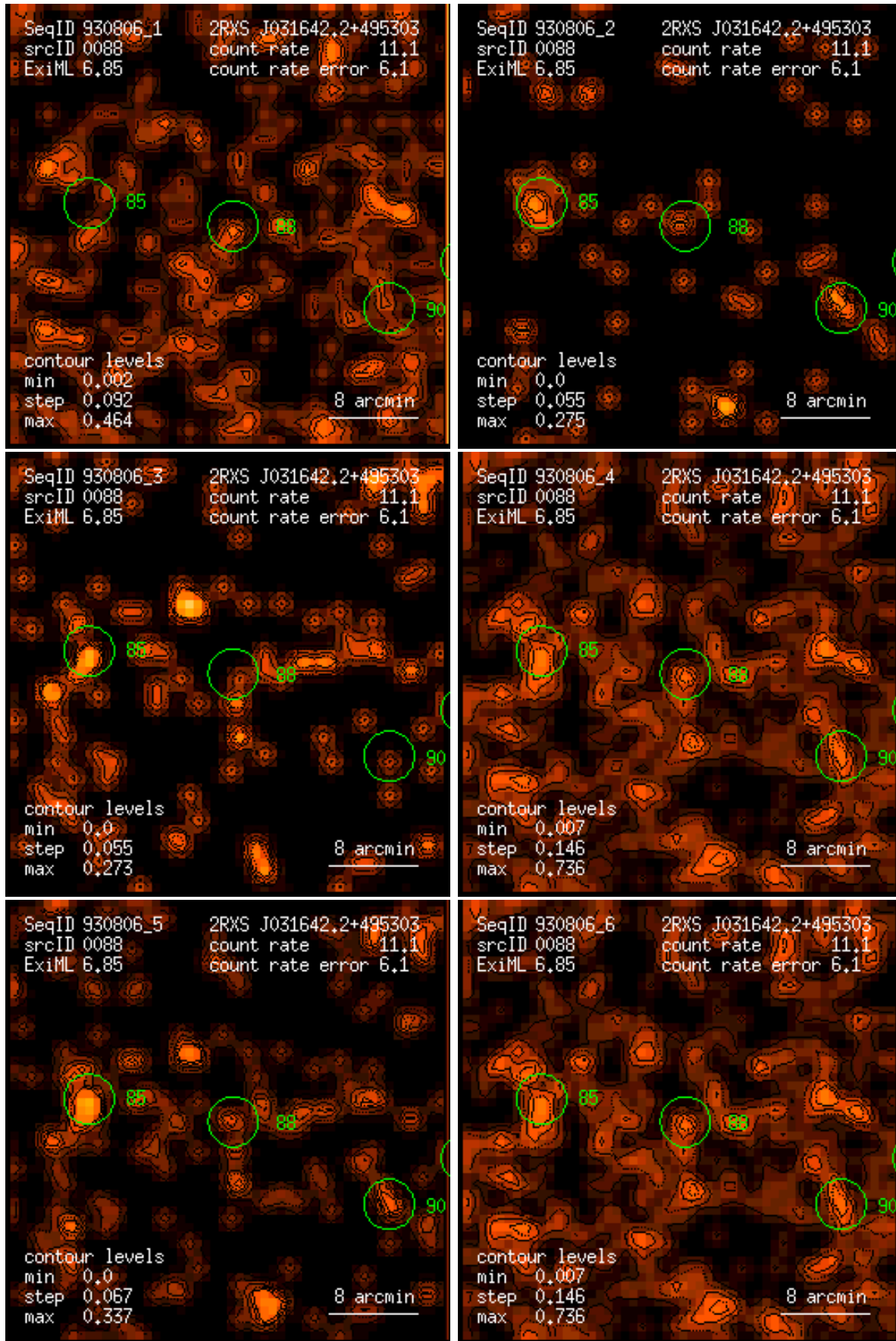
Figure 88: RASS 930806: detection 0088: band rate images, Gaussian filter: (1) PSPC channels 11 – 41, (2) 52 – 90, (3) 91 – 201, (4) 11 – 235, (5) 52 – 201, (6) 11 – 201. Broad band rates in counts/ks. Band rate contour levels in counts/ks/arcmin 2 .
