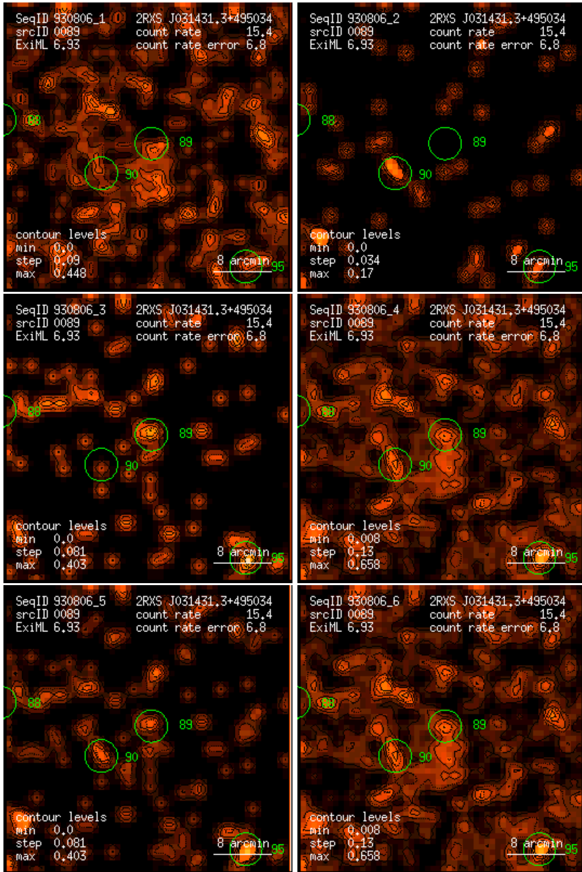
Figure 89: RASS 930806: detection 0089: band rate images, Gaussian filter: (1) PSPC channels 11 – 41, (2) 52 – 90, (3) 91 – 201, (4) 11 – 235, (5) 52 – 201, (6) 11 – 201. Broad band rates in counts/ks. Band rate contour levels in counts/ks/arcmin 2 .
