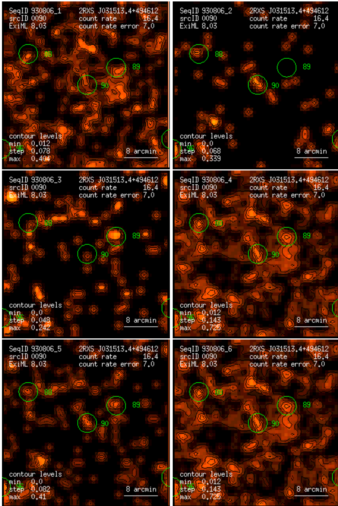
Figure 90: RASS 930806: detection 0090: band rate images, Gaussian filter: (1) PSPC channels 11 – 41, (2) 52 – 90, (3) 91 – 201, (4) 11 – 235, (5) 52 – 201, (6) 11 – 201. Broad band rates in counts/ks. Band rate contour levels in counts/ks/arcmin 2 .
